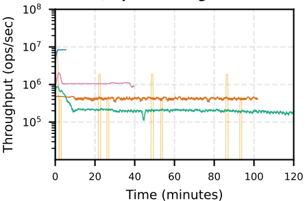
a) Updates on g500-24
