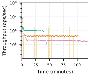
(c) Updates on g500-24
