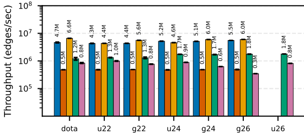
(b) Insertion throughput
