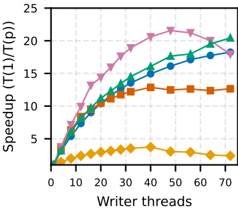
(a) Scalability
