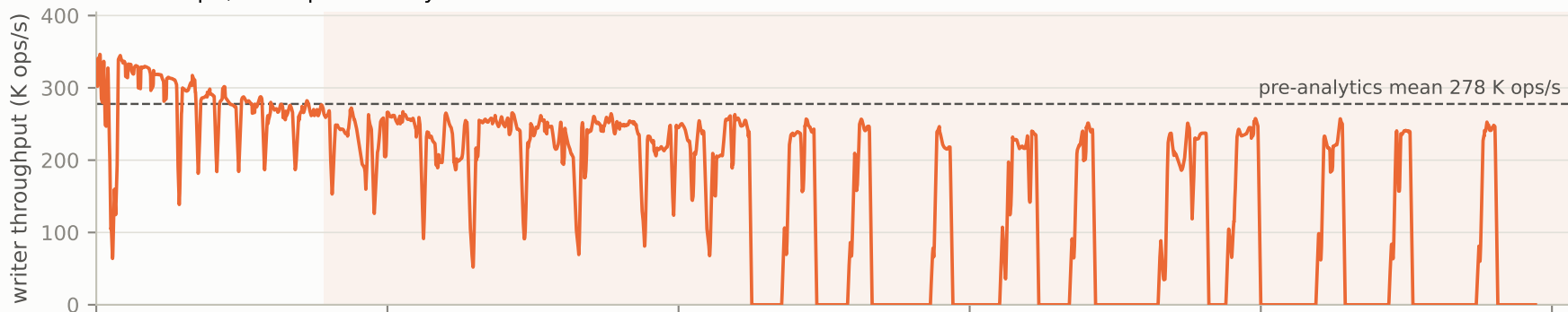
LiveGraph, in memory
