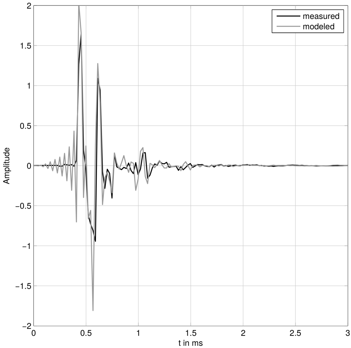
Left ear HRIR
