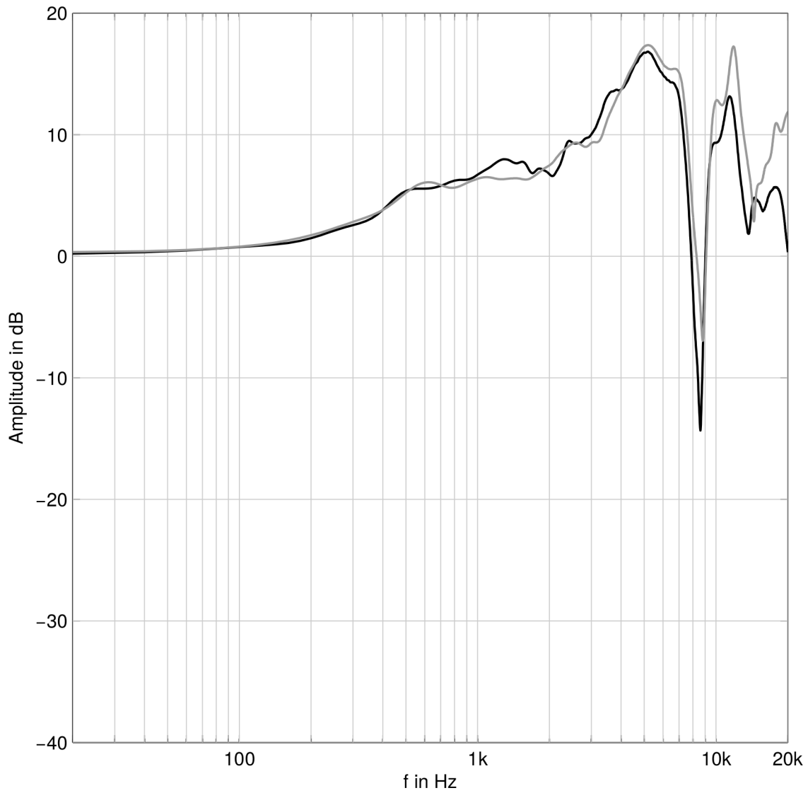
Left ear HRTF
