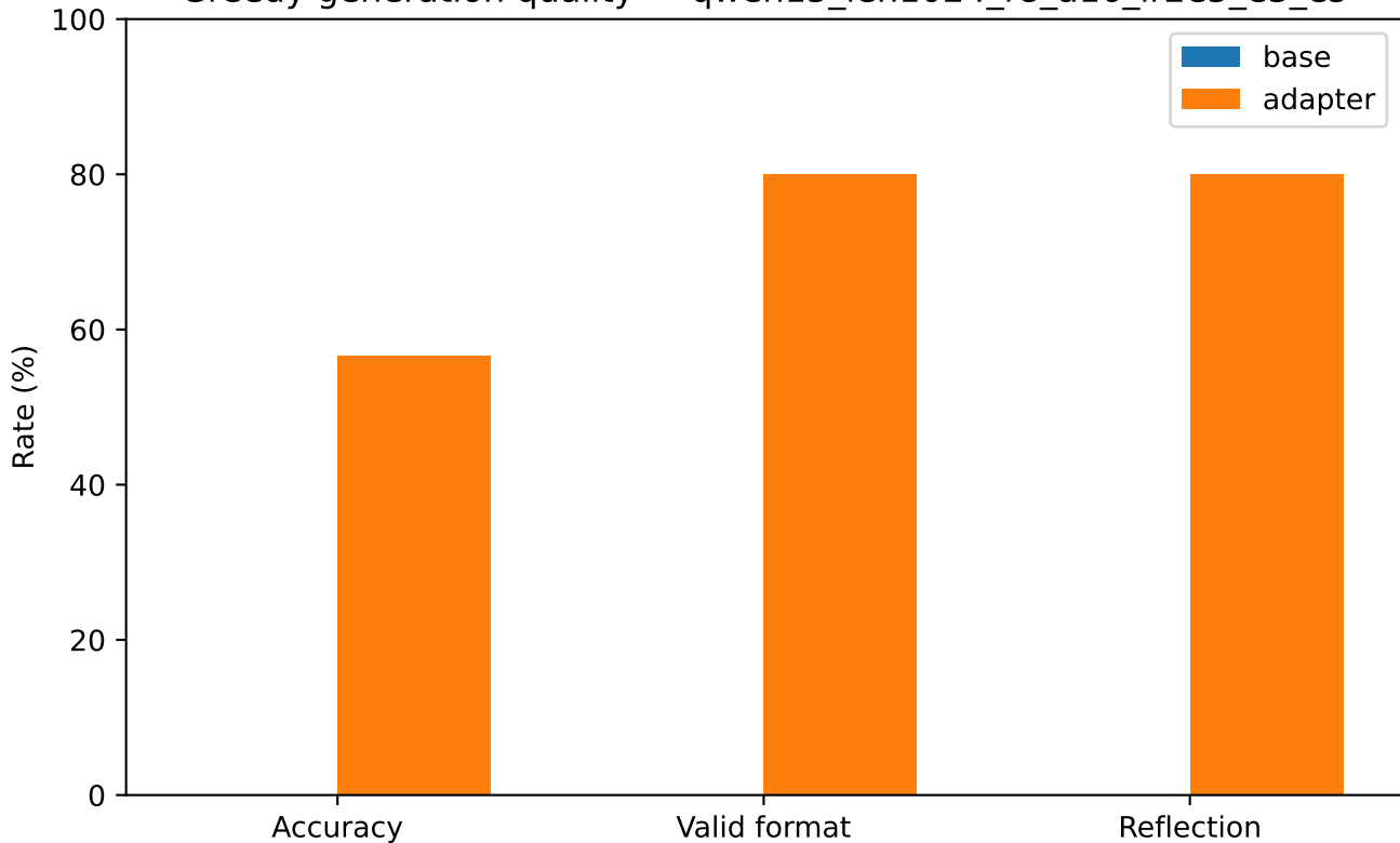
Greedy generation quality — qwen15_len1024_r8_a16_lr2e5_e3_es
