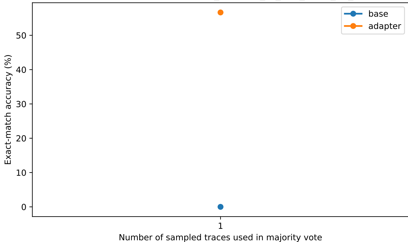
Self-consistency — qwen15_len1024_r8_a16_lr2e5_e3_es
