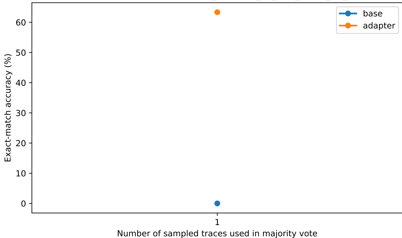
Self-consistency — qwen15_len1024_r8_a16_lr5e5_e3_es
