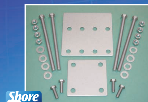
Deck Mounting Hardware One 5", 8-Hole Plate, Four 3/8" x 6" Bolts with Washers & Nuts and One Leveling Kit
