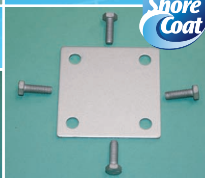
Leveling Kit One 3.5", 4-Hole Plate and Four 4 1/4" x 1" Leveling Screws
