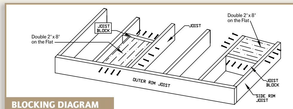
BLOCKING DIAGRAM
