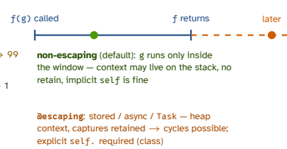
C Escaping = outlives the call
