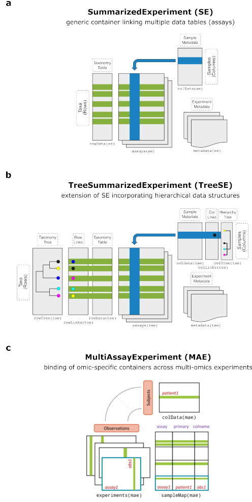
Figure 2: Integrative Bioconductor containers for microbiome data. (a) SummarizedExperiment (SE) 28 is a generic container for single-omics experiments. It accommodates assays that describe the feature abundances in each sample ( e.g. , taxonomic units, resistance genes, or predicted functions), and tabular side information on each sample ( colData ) and feature ( rowData ), e.g. , the taxonomic classification. (b) TreeSummarizedExperiment (TreeSE) 30 supports hierarchical, multi-table microbiome analysis. In addition to the SE elements, TreeSE incorporates tree information on feature hierarchies, such as phylogenetic relations between the taxonomic units ( rowTree ) or host species ( colTree ), and results of dimensionality reduction ( reducedDims ). TreeSE can thus link multiple abundance tables and their transformed versions ( e.g. , statistical transformation, taxonomic agglomeration, or dimensionality reduction) with tabular and hierarchical side information on the features (rows) and samples (columns). Additional slots for reference sequences and experiment metadata are available. (c) MultiAssayExperiment (MAE) 31 facilitates the integration of interlinked datasets representing different omics modalities linked by potentially non-trivial sample mappings. Figure adapted from 31 .
