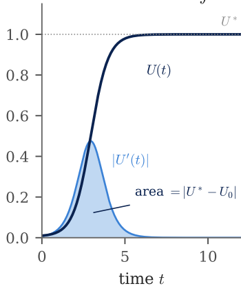
(a) U is monotone, \int |U'| < \infty
