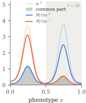
(c) the overlap cancels
