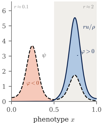
(b) forcing \varphi = U'(ru/\rho - \psi)
