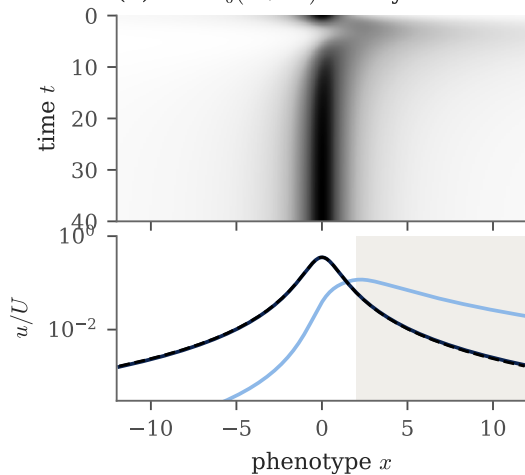
(b) D = D_0(1 + x^2) : heavy tails
