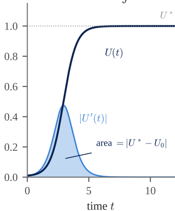
(a) U is monotone, \int |U'| < \infty
