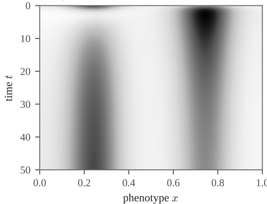
(e) total population U
