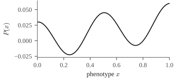
(c) u/U , uniform competition
