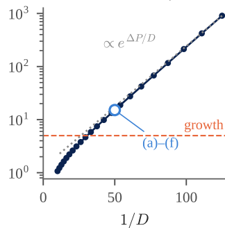
(g) memory time 1/\lambda_1
