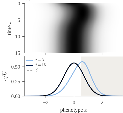
(a) Ornstein–Uhlenbeck on \mathbb{R}
