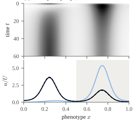
(c) Metropolis jumps, no diffusion
