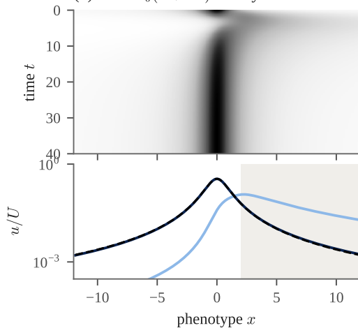
(b) D = D_0(1 + x^2) : heavy tails
