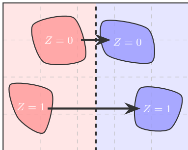
Group regularization
