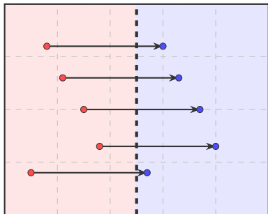
Individual regularization
