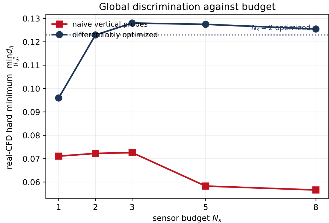
Real CFD: sensor placement versus sensor count (no new CFD, same 66-angle bank)
