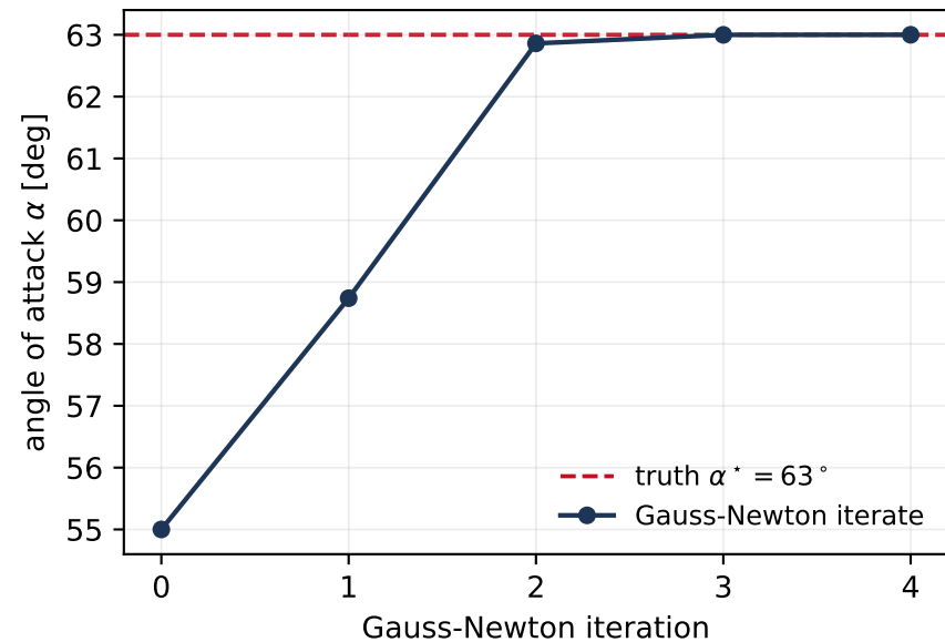
Recovered angle of attack
