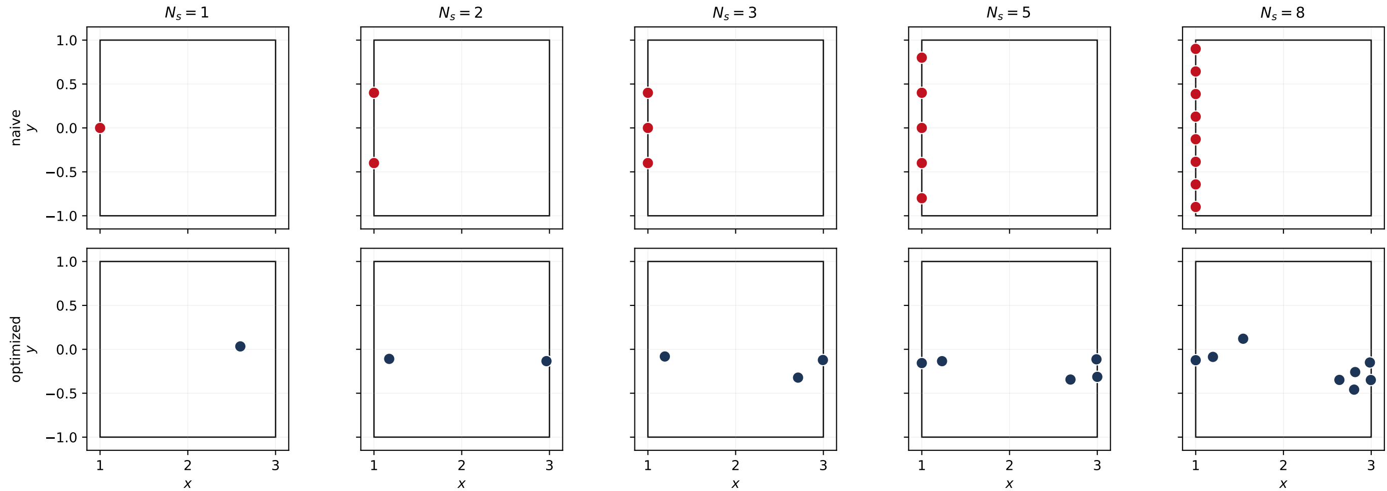
Probe layouts: conventional vertical array versus optimized
