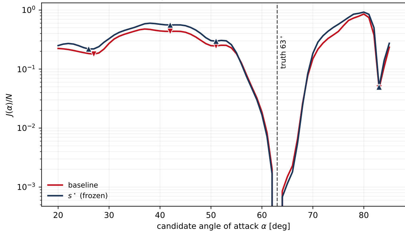
Real-CFD inverse landscape at the sealed truth (markers: false local minima)
