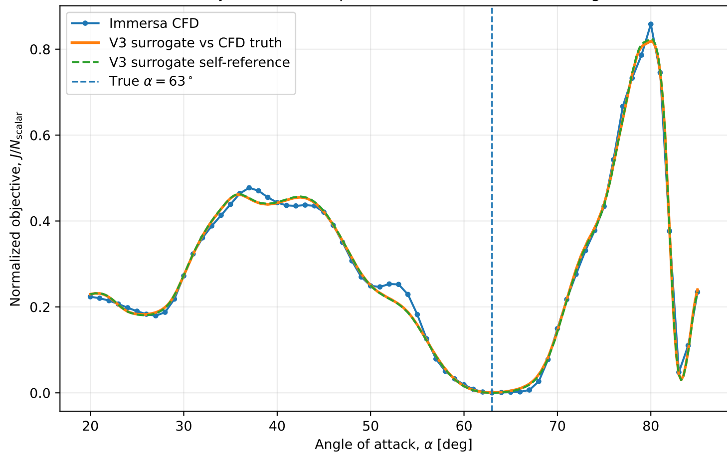
Inverse-objective landscape: Immersa CFD vs WakeSurrogate V3
