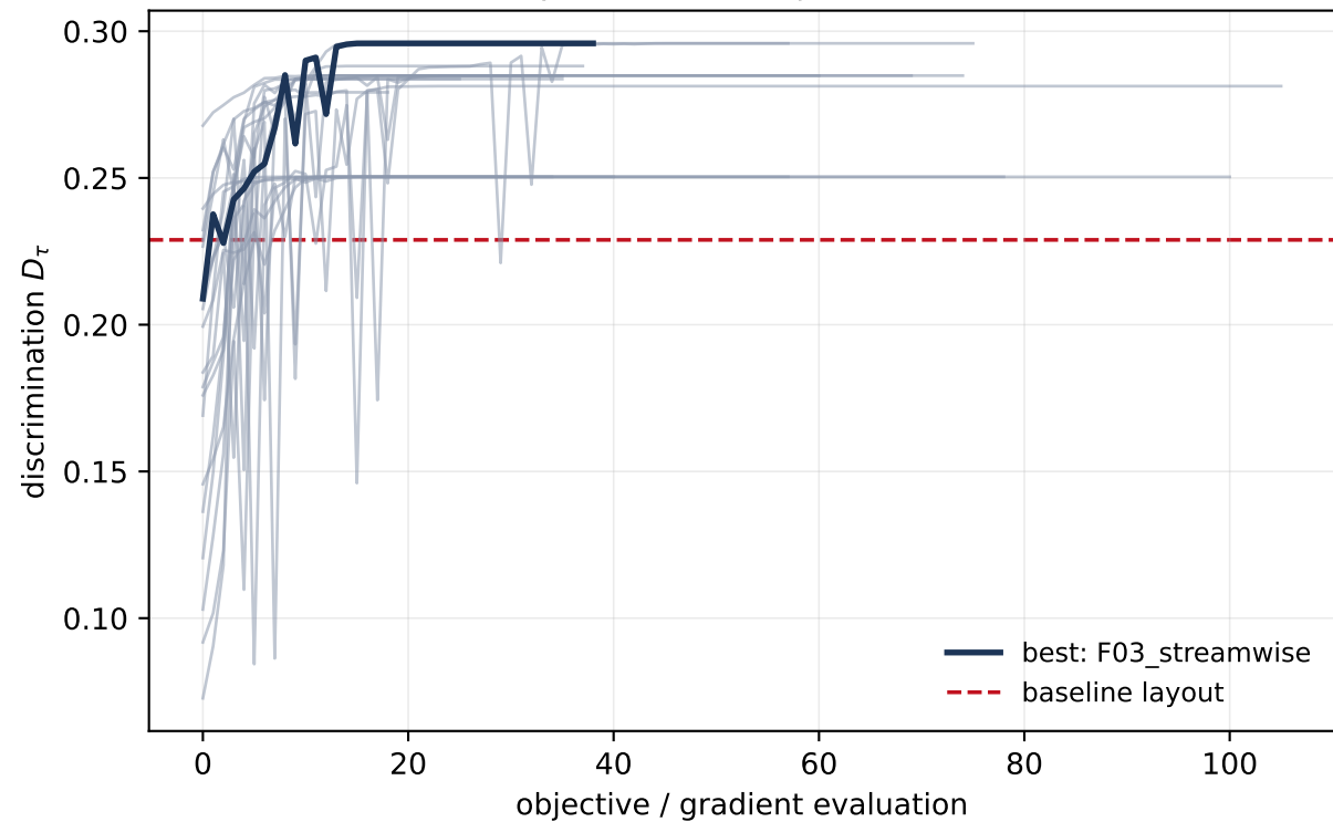
Multistart optimization trajectories (20 starts)
