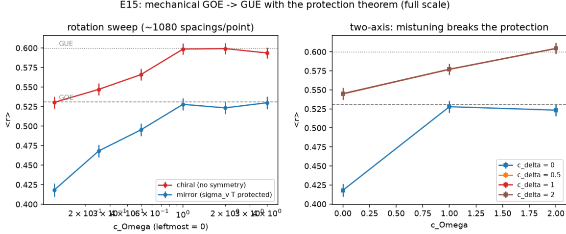
Figure 8: E15 at full scale. Left: rotation sweep — the chiral rotor crosses \text{GOE} \rightarrow \text{GUE} while the \sigma_v T -protected mirror rotor saturates at GOE. Right: mistuning breaks the protection; rotation and mistuning together reach GUE.
