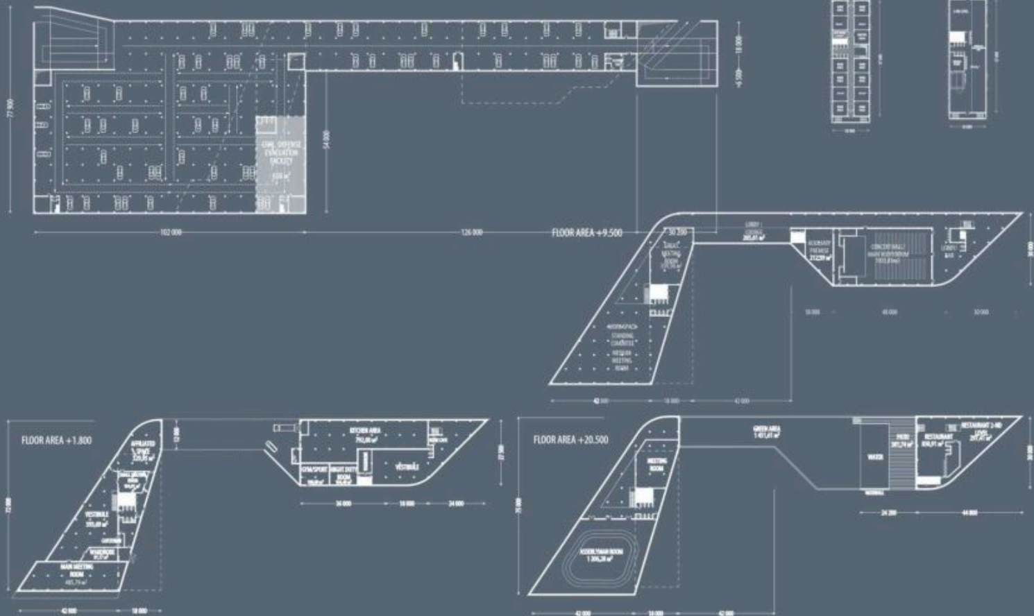
UNDERGROUND PARKING FLOOR PLAN - 1.500
