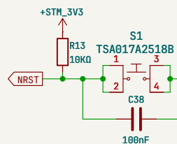
RESET TACTILE SWITCH
