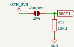
BOOT1 SELECTOR
