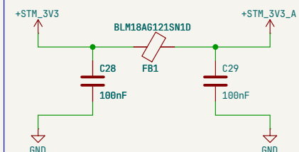
ANALOG FILTERING
