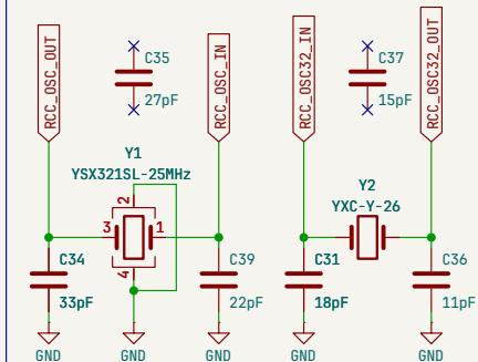
HSE CRYSTAL
