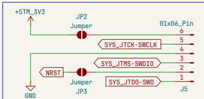
ST-LINK DEBUGGER AND FLASHING
