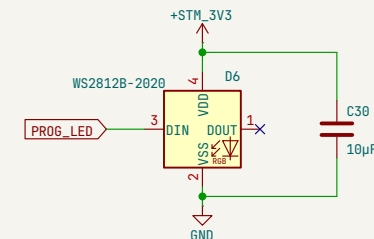
PROGRAMABLE RGB LED
