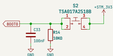
BOOT TACTILE SWITCH
