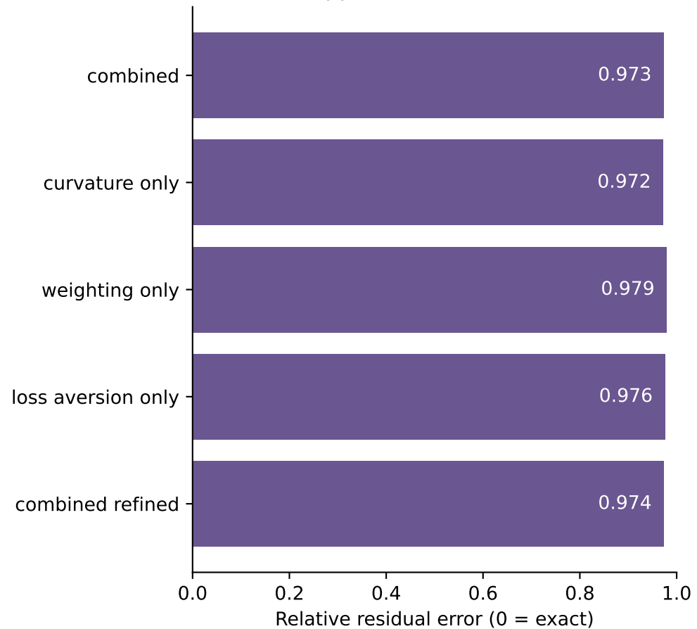
Ten-feature approximation of LoRA mean shift
