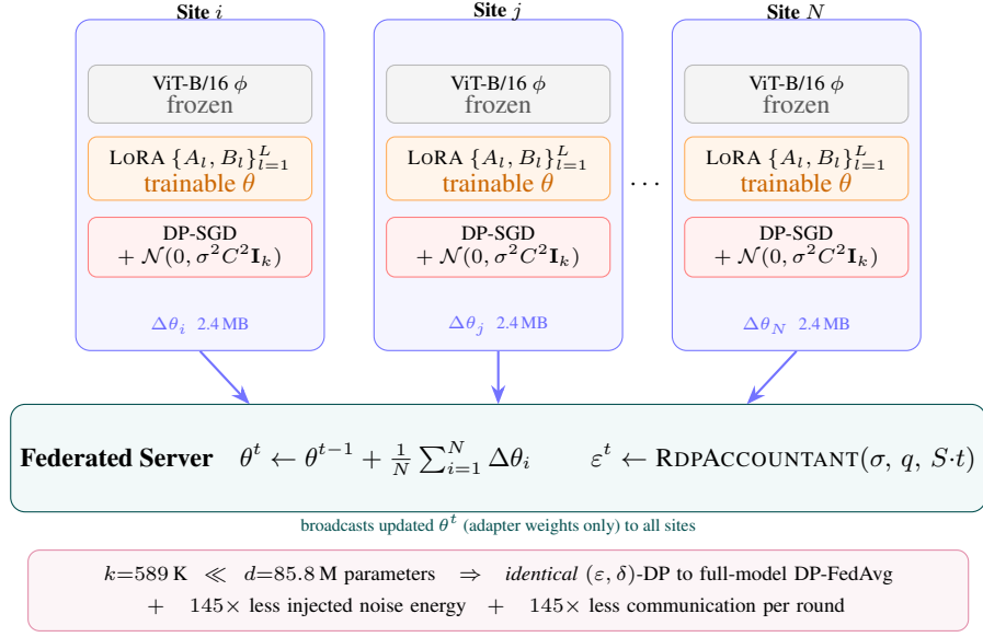
Figure 1: DP-FedLoRA system overview. Each of N hospital sites freezes the ViT-B/16 backbone ( \phi , d=85.8\text{M} parameters) and trains only the LoRA adapter matrices \theta=\{A_l, B_l\}_{l=1}^L ( k=589\text{K} parameters, 0.69\% of d ). Opacus DP-SGD computes per-sample gradients and adds Gaussian noise \mathcal{N}(0, \sigma^2 C^2 \mathbf{I}_k) to adapter gradients only before upload; the frozen backbone receives no noise. Each site uploads a 2.4 MB adapter delta (versus 343 MB for full-model DP), which the server aggregates via FedAvg. Privacy is tracked per round using the RDP moments accountant and composed across all T rounds. Because k \ll d , DP-FedLoRA achieves the same (\varepsilon, \delta) -differential privacy as full-model DP-FedAvg at identical \sigma , C , q , S while injecting 145\times less noise energy and transmitting 145\times less data per round (Theorem 1; Proposition 1).
