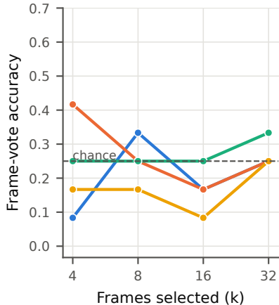
All questions (n=12)
