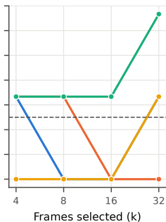
Perception (n=3)
