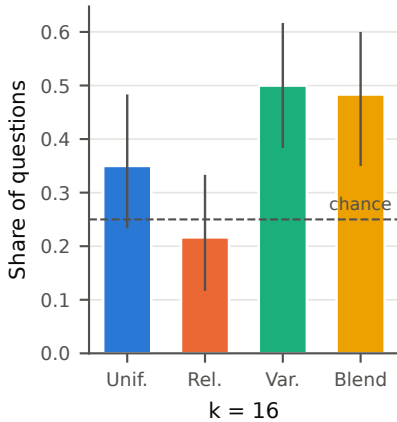
(b) Votes for text odd-one-out
