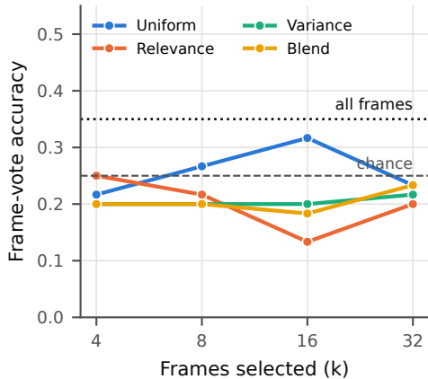
(a) Vote accuracy (n=60)
