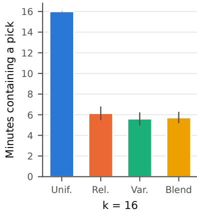
(c) Distinct minutes hit
