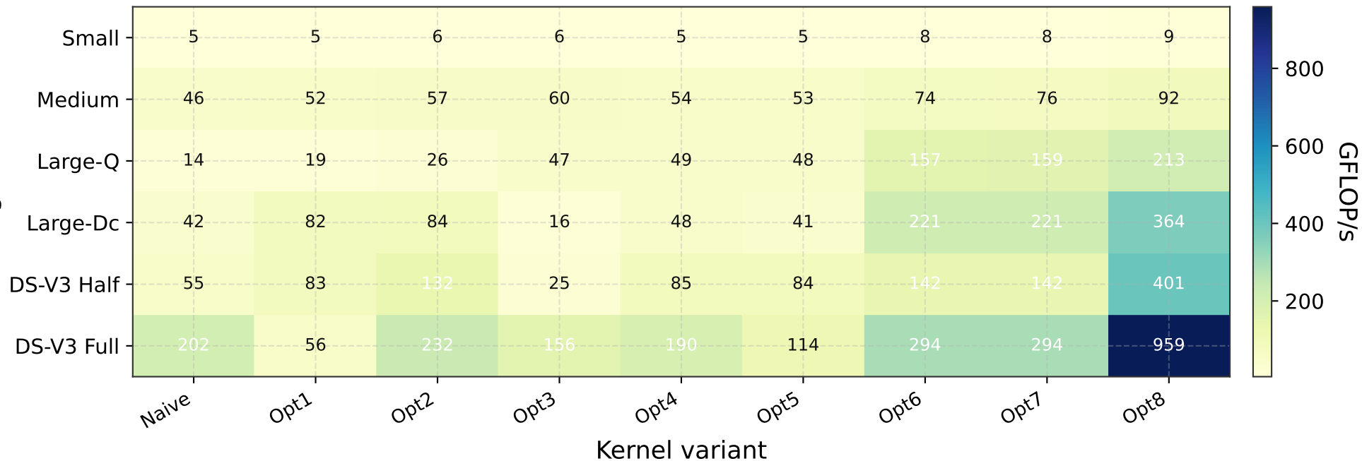
DSA kernel variants (bench_dsa_full) — GFLOP/s heatmap
