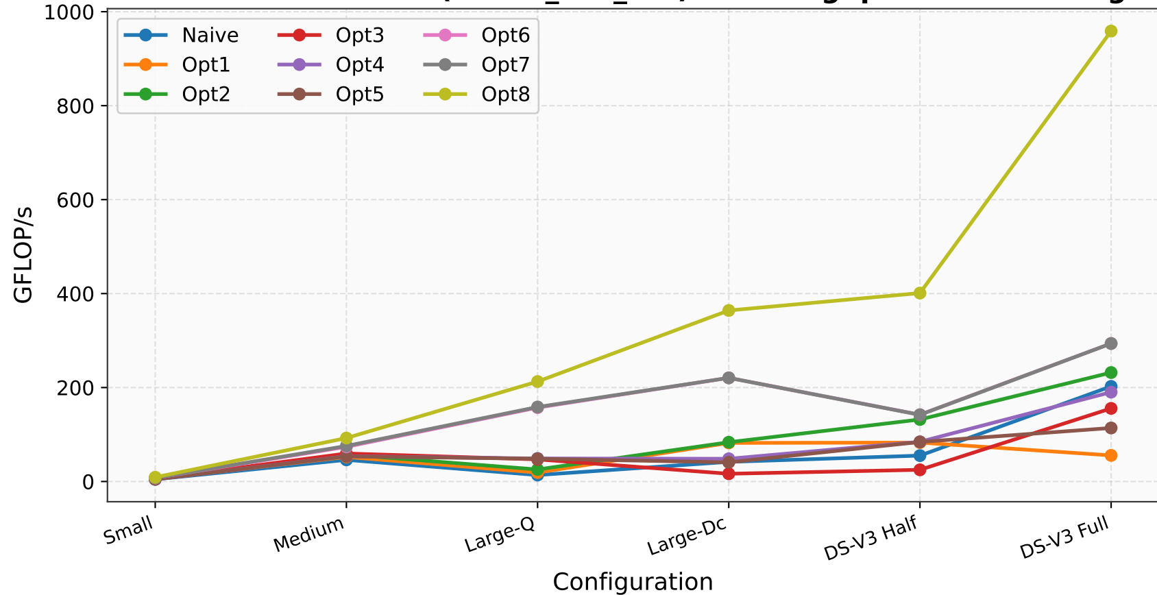
DSA kernel variants (bench_dsa_full) — throughput across configs
