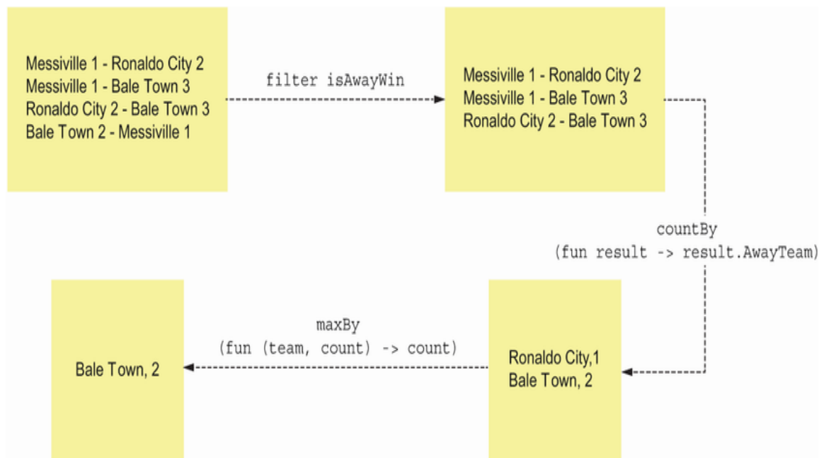
Figure 7.2 Visualizing the data transformations within a pipeline
