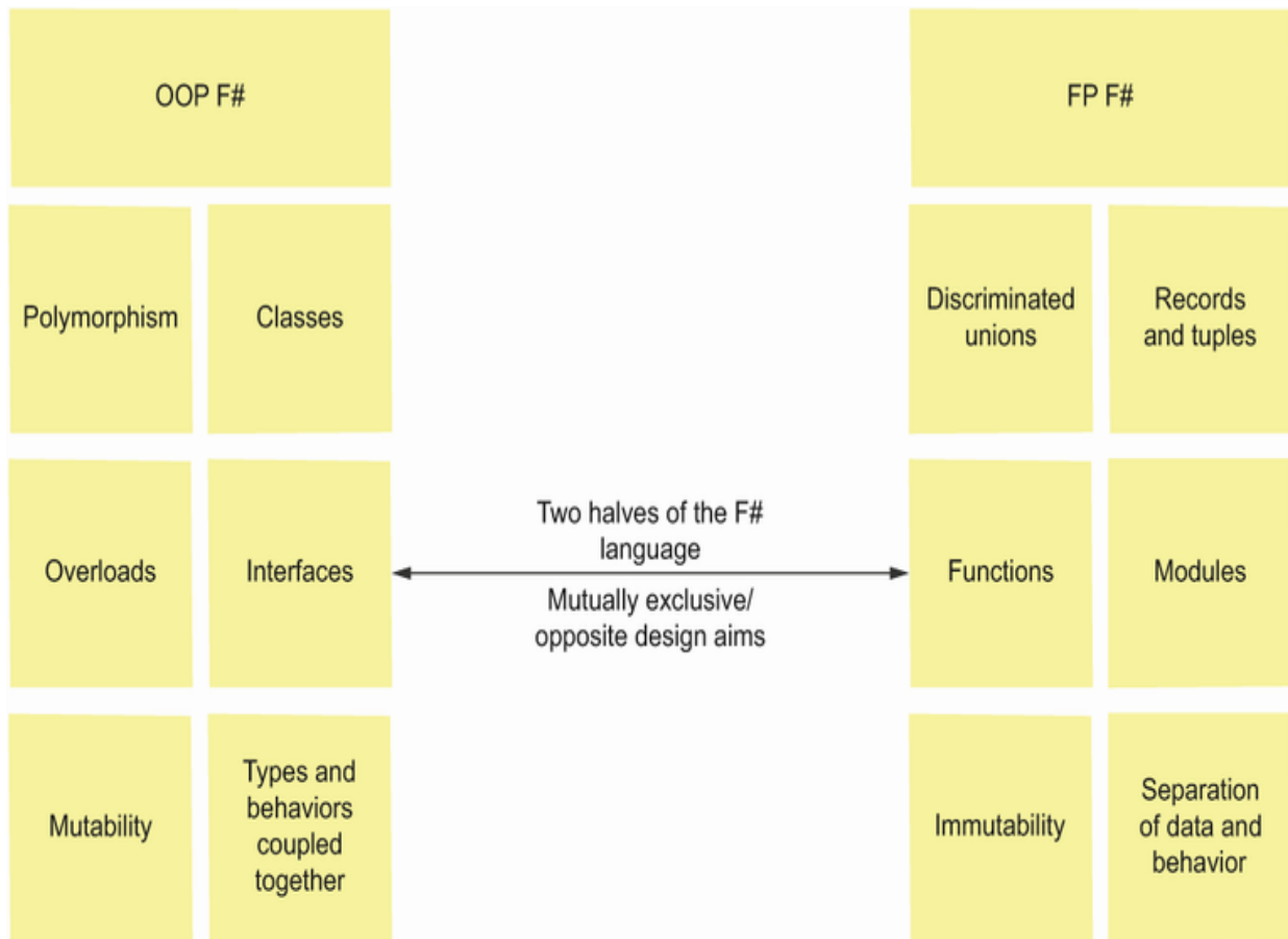
Figure 11.1 Illustrating the clear distinction between the object orientated (OO) and functional programming (FP) halves of F#
