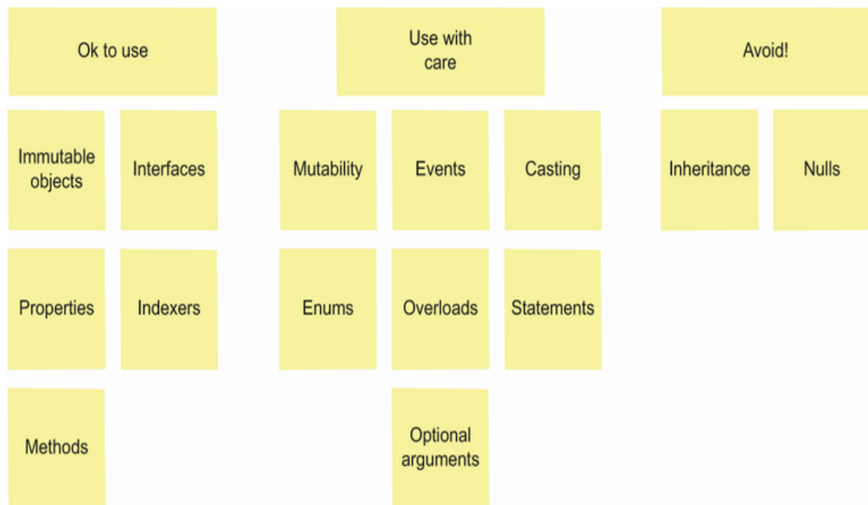
Figure 11.2 Some of the different OO features in F#. Many of these can be happily used in idiomatic F#, but others should be avoided except where necessary.
