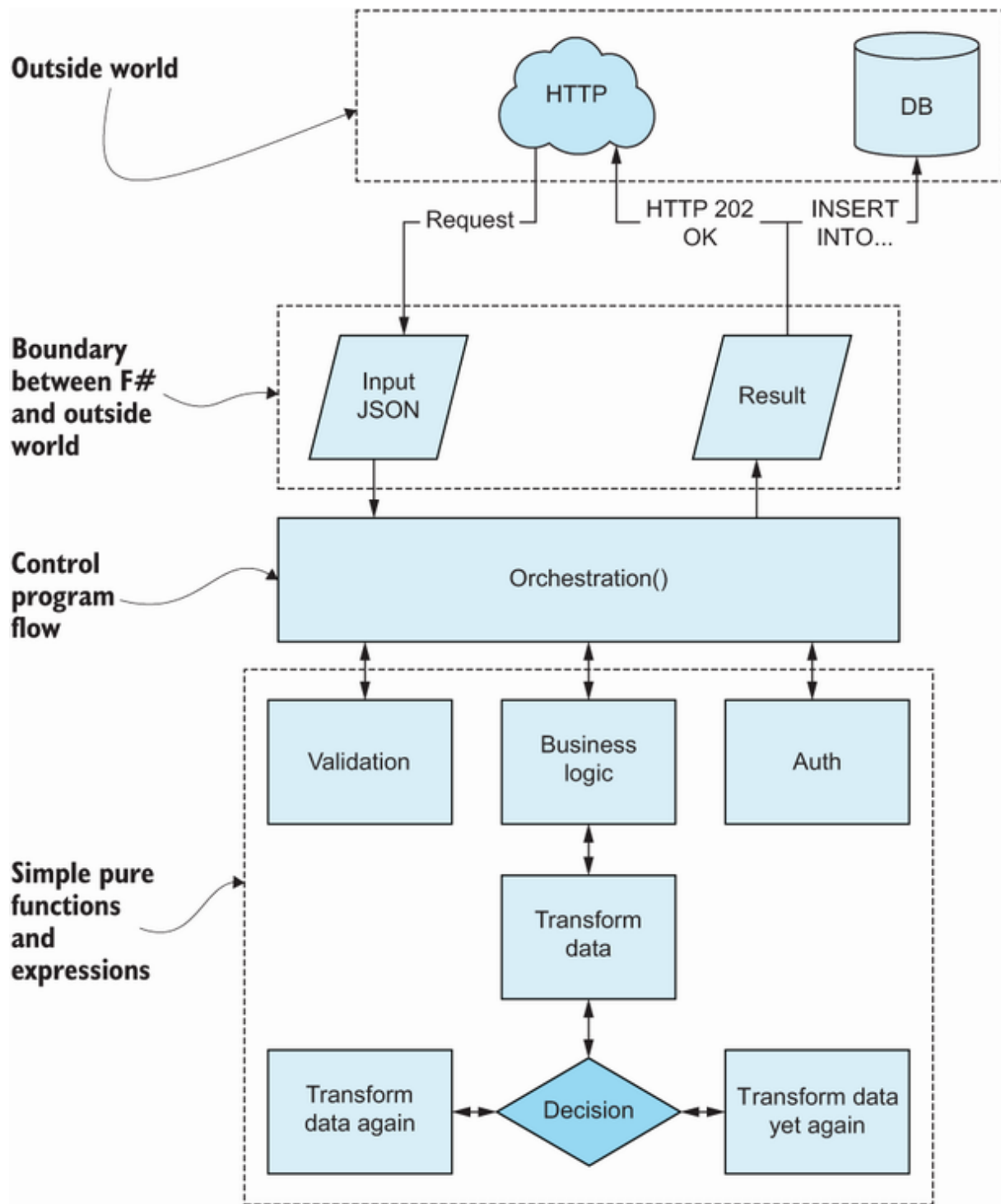
Figure 15.1 A fictional expression chain of function calls, with separation between the impure outside and (mostly) pure inner world
