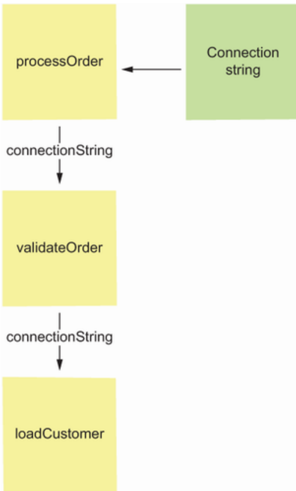
Figure 15.3 Passing a low-level implementation argument through a top-level function can cause extra coupling and complexity throughout your code.
