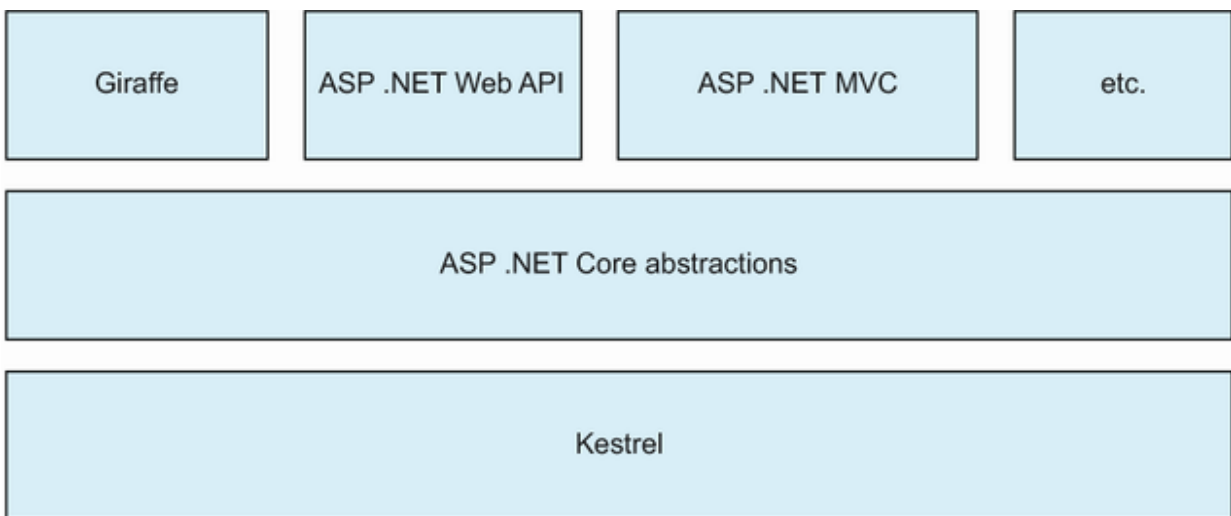
Figure 13.2 The ASP.NET Core stack contains a low-level, high-performance web server called Kestrel, upon which core abstractions exist. Finally, developer-level frameworks exist, such as MVC and Giraffe.
