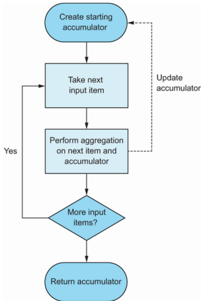
Figure 7.8 Visualizing a typical generic aggregation algorithm
