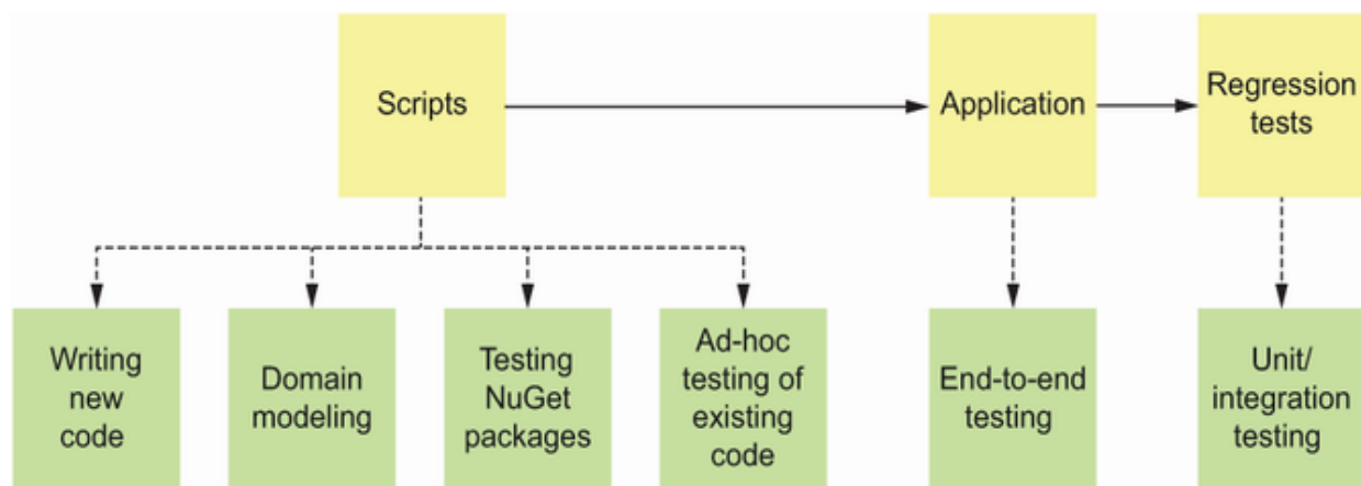
Figure 2.4 The different types of uses for F# scripts
