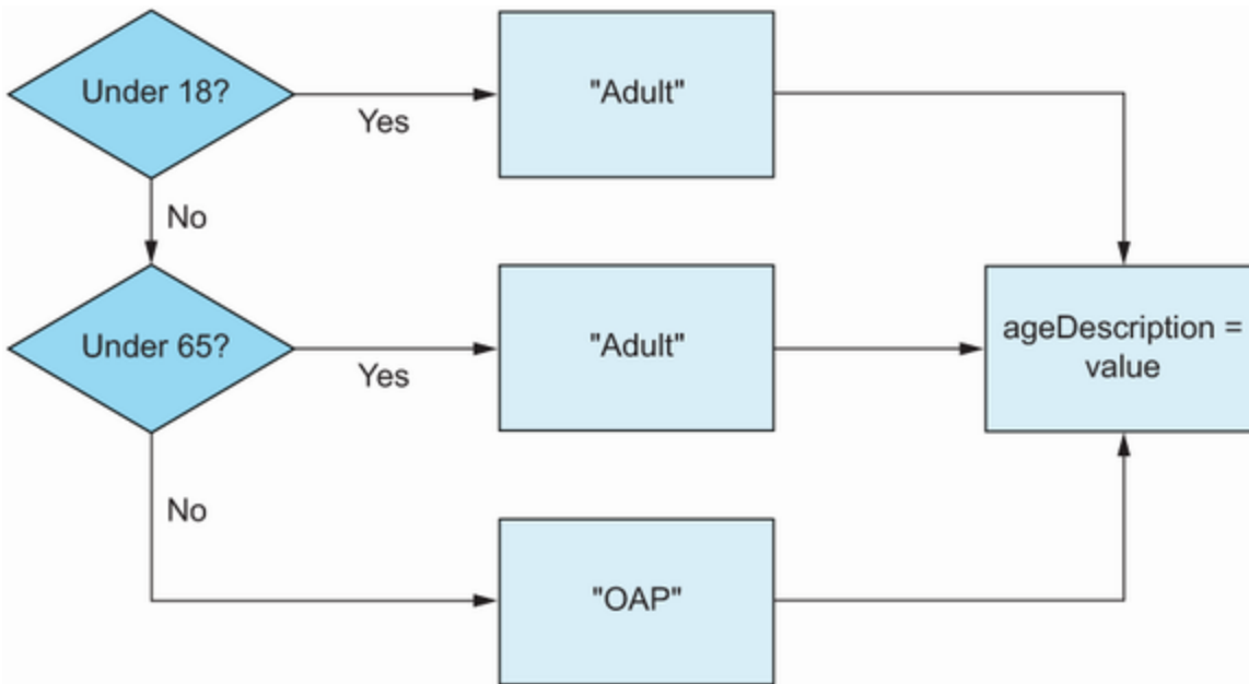
Figure 4.2 Expressing the same flow but using expressions
