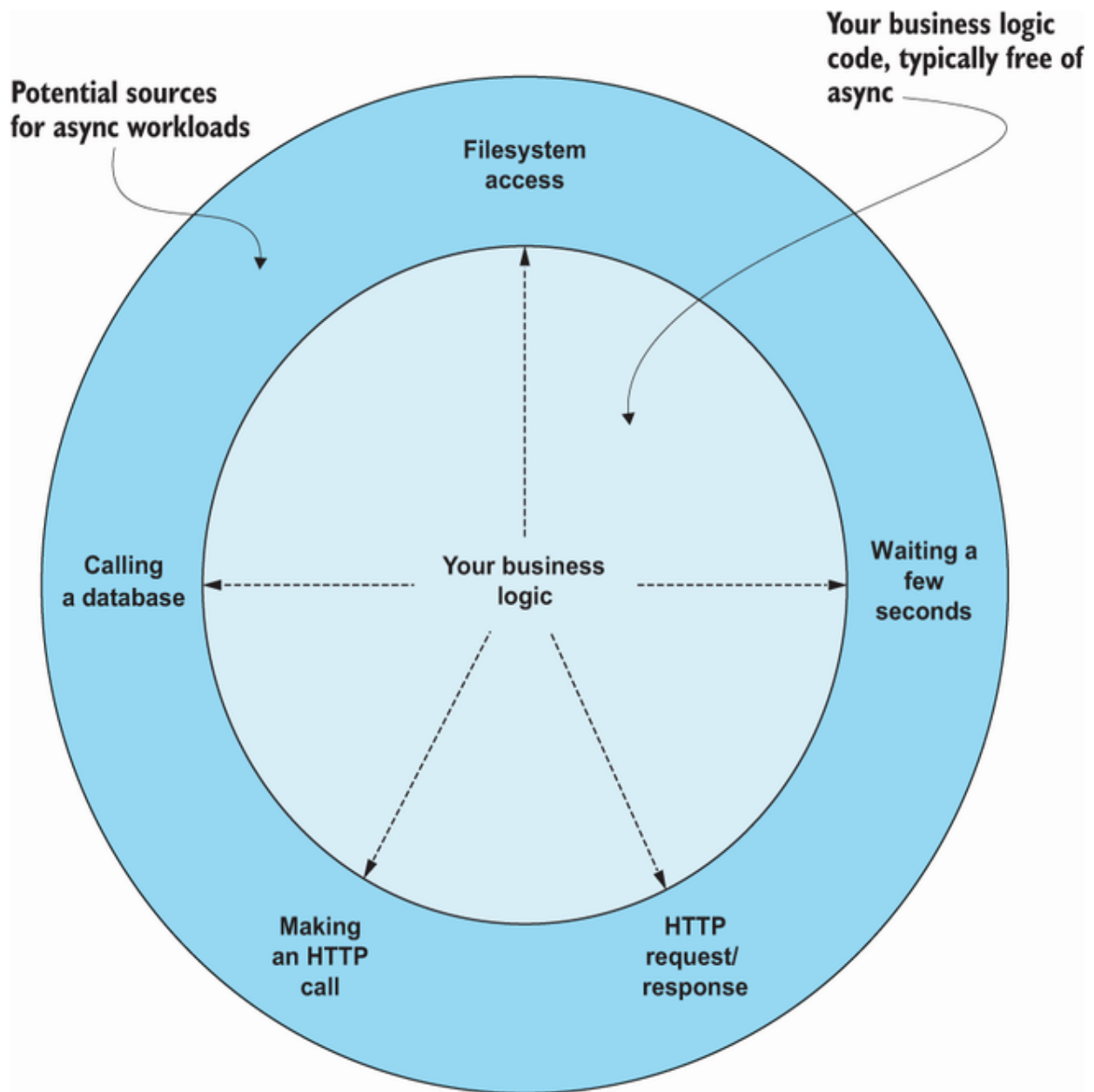
Figure 12.2 Most I/O operations will have asynchronous APIs; your business logic will typically be synchronous in nature, but the boundaries of your application will introduce asynchronous operations, which you can compose together using task { } blocks.
