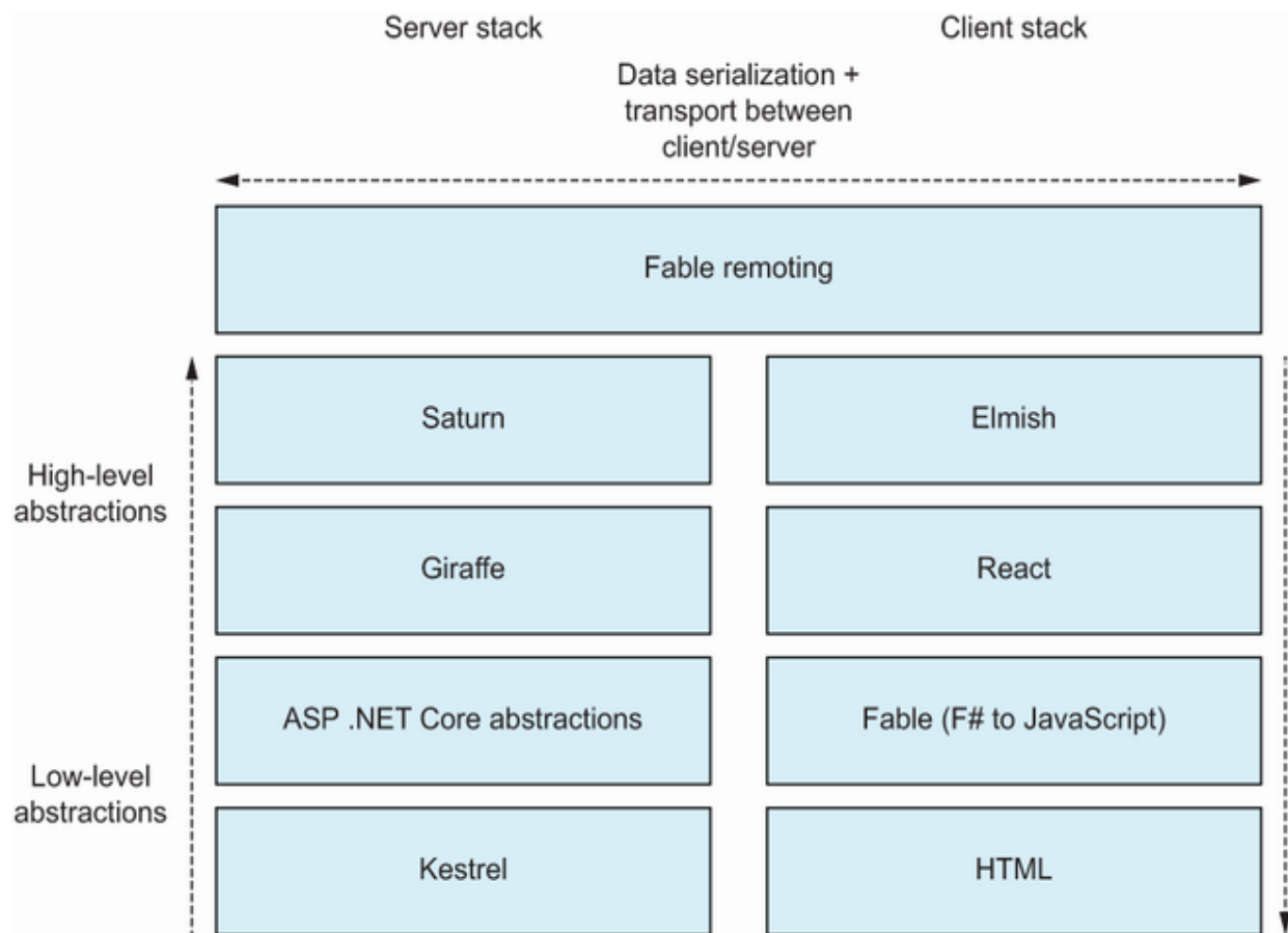
Figure 13.12 The SAFE Stack is a collection of different technologies bundled together to allow writing standards-compliant, rich web applications entirely in F#. The left-hand side of this figure represents the server side of the stack; the right-hand side represents the client side, which typically runs in the browser as a so-called single-page application.
