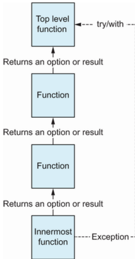
Figure 9.4 Options and results are normal return values of functions, whereas an exception can implicitly bubble all the way up the call stack until it encounters a try/with block.
