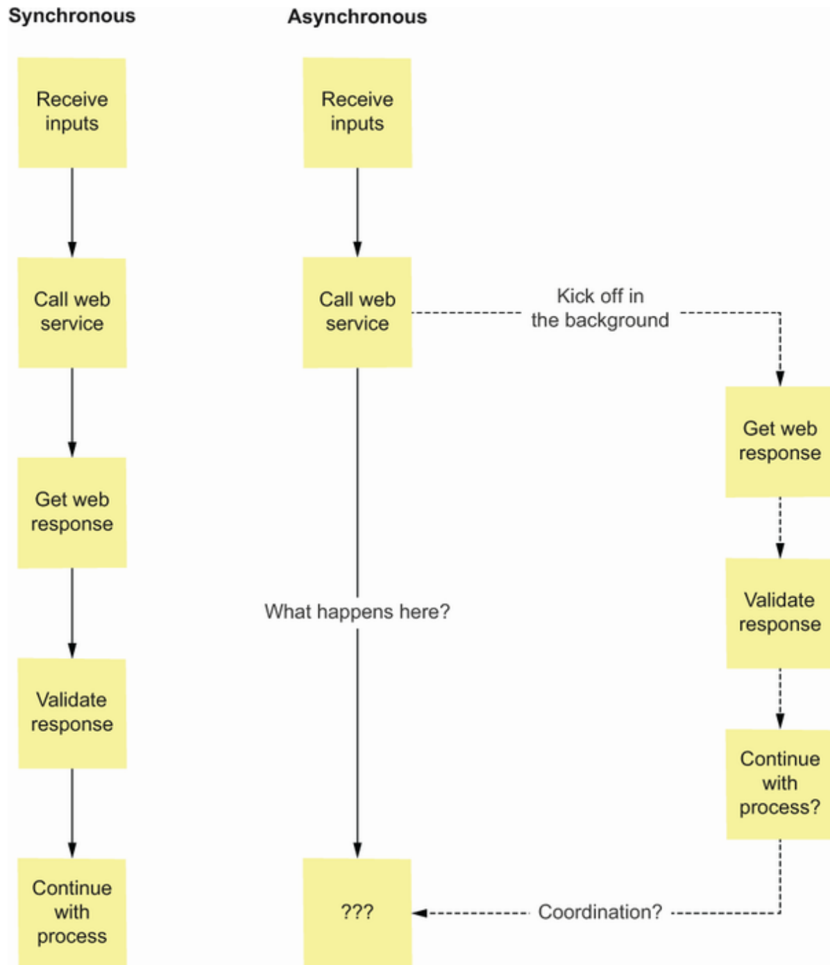
Figure 12.1 Comparing synchronous and asynchronous flows. The synchronous flow follows a single, sequential flow. The asynchronous flow branches into two streams, which requires
