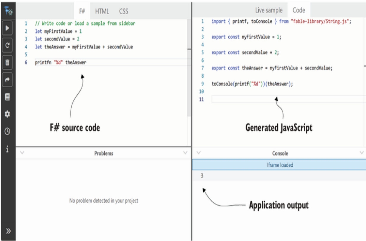
Figure 11.6 The Fable REPL in action. F# entered on the upper-left pane is converted into JS and then run. The output in the bottom-right pane shows any console output.
