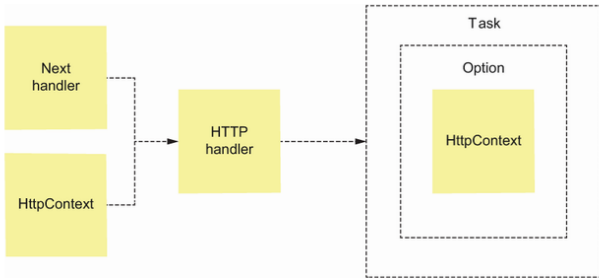
Figure 13.7 The HTTP Handler signature represented graphically. The two inputs are the next handler in the pipeline (called the HttpFunc ) and the HTTP Context. The Handler must asynchronously return either nothing or Some context. This can be done itself or by delegating the result to the next handler.
