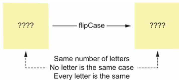
Figure 14.3 Testing a function by proving that for any given input, it exhibits a set of rules or properties that govern the relationship between the input and output
