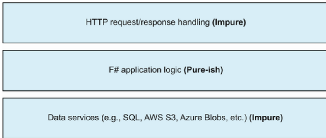
Figure 13.9 Visualizing a web application through the prism of pure/impure layers. F# code should favor purity where it's possible and not overly complicated to achieve.
