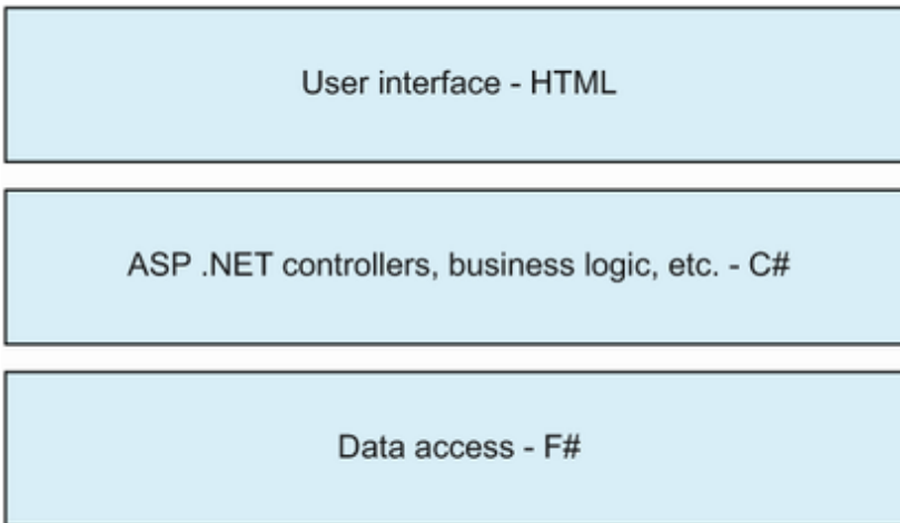
Figure 11.3 A horizontal tiers approach to introducing F# into a mixed-language application. Here, F# is used for all data access operations but is called from a C# layer on top.
