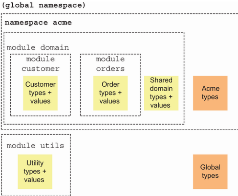
Figure 6.4 Namespaces and modules in a single application
