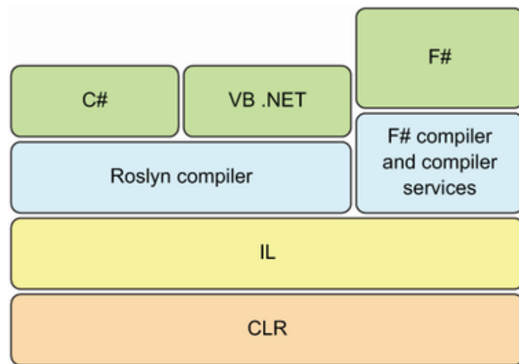
Figure 2.1 A simplified view of the .NET language and runtime landscape
