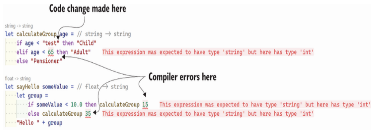
Figure 3.4 Type Inference behaving in a way that may be unexpected
