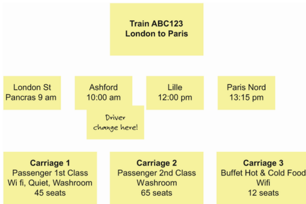
Figure 9.7 An example train manifest that needs to be modeled in F#
