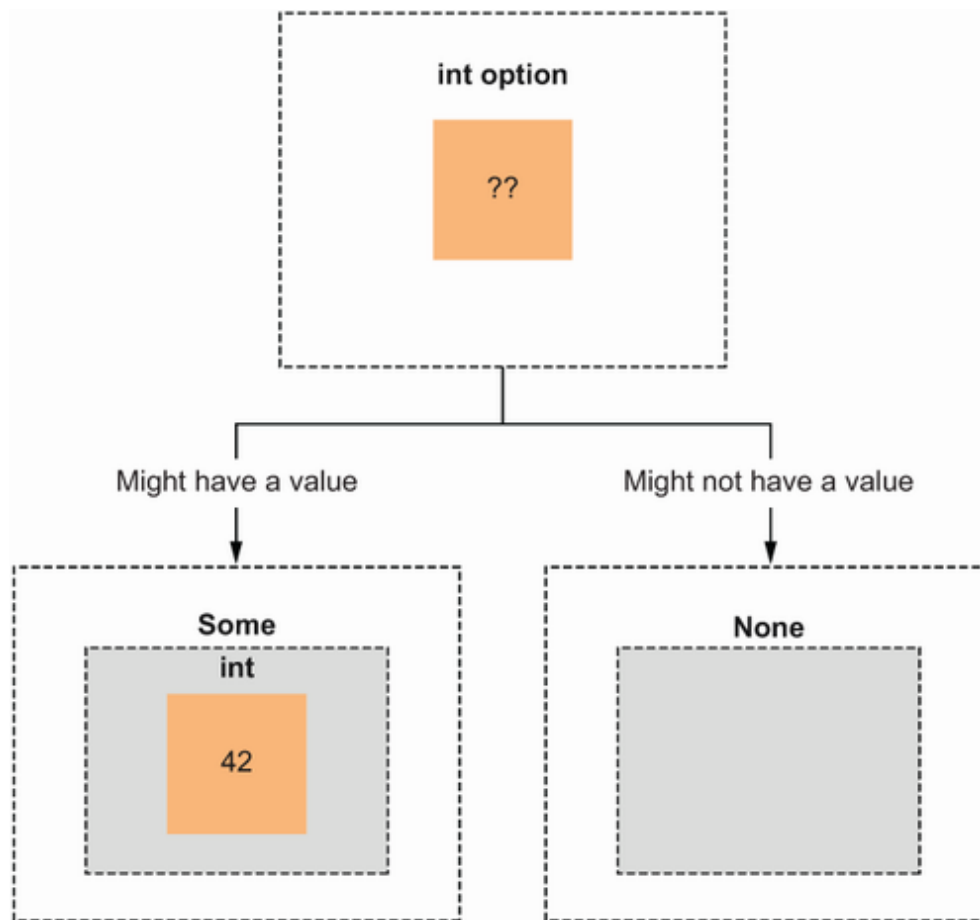
Figure 9.1 Unlike an int , an int option can have two outcomes: either it wraps a real int , or it has nothing in it. You need to pattern match on the value to safely check whether there's data inside it and then proceed accordingly.
