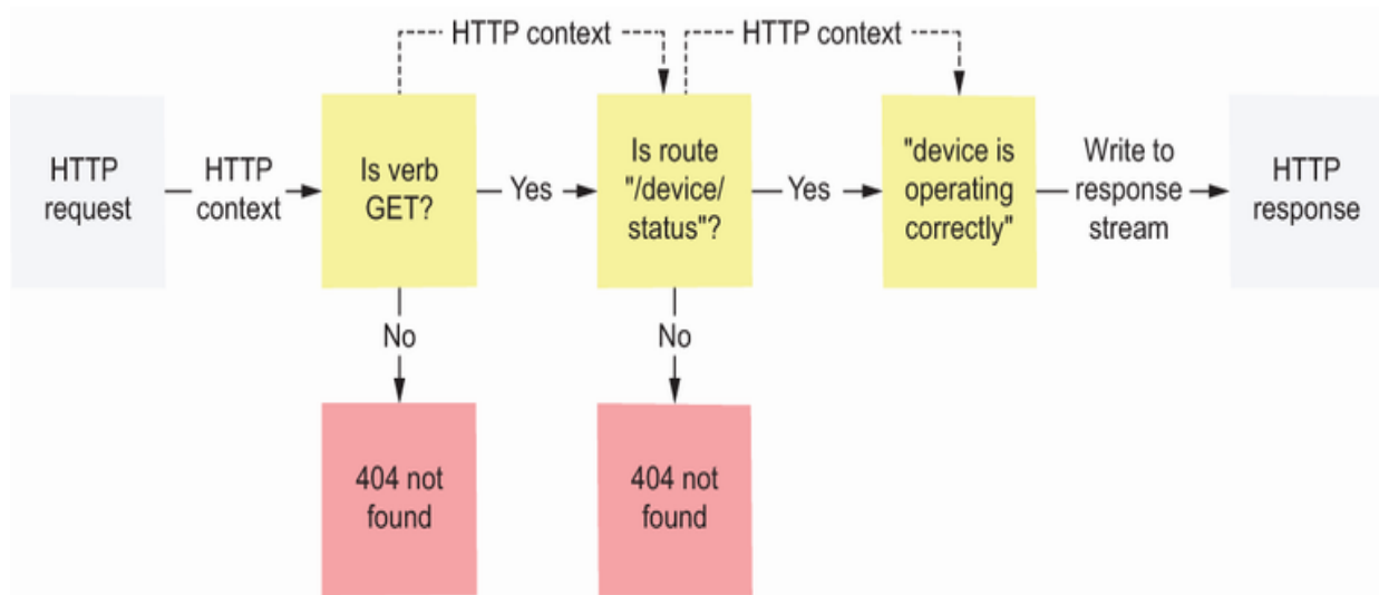
Figure 13.6 The same HTTP request/response as figure 13.5, except shown as a Giraffe pipeline. The central three cards represent three HTTP Handlers that each fulfill a specific purpose. The first two act as filters; the last one writes to the response stream.
