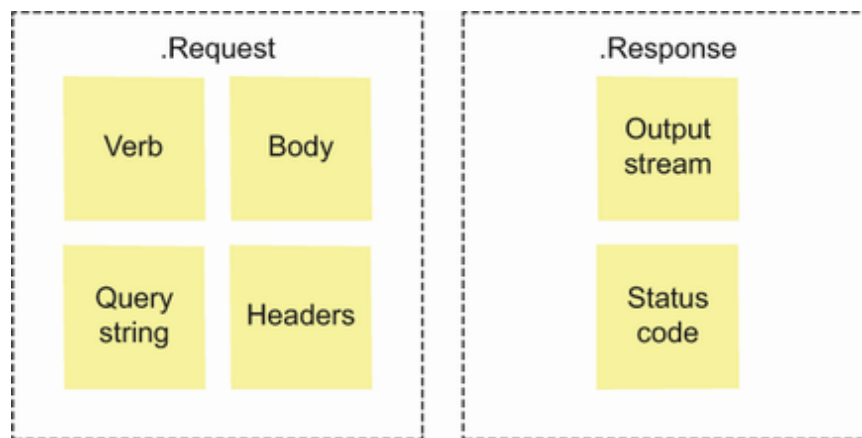
Figure 13.4 The HTTP Context contains properties such as .Request and .Response , in which you can access data that directly represents the incoming and outgoing HTTP messages.
