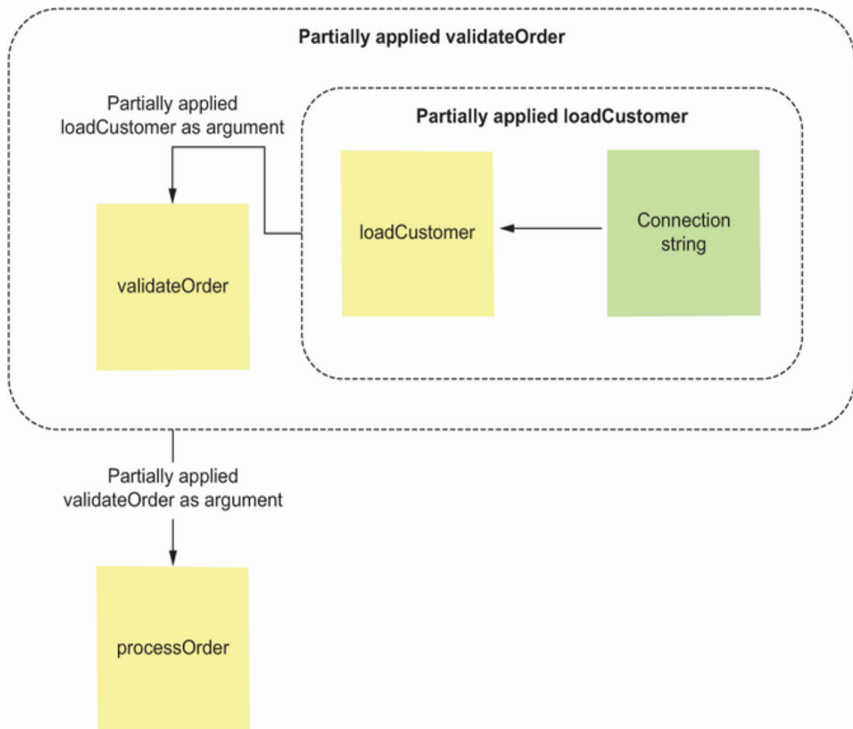
Figure 15.4 A bootstrapper function inverts dependencies and uses partial application to allow you to supply preconfigured, low-level functions to your top-level code, avoiding the challenges shown in figure 15.3.
