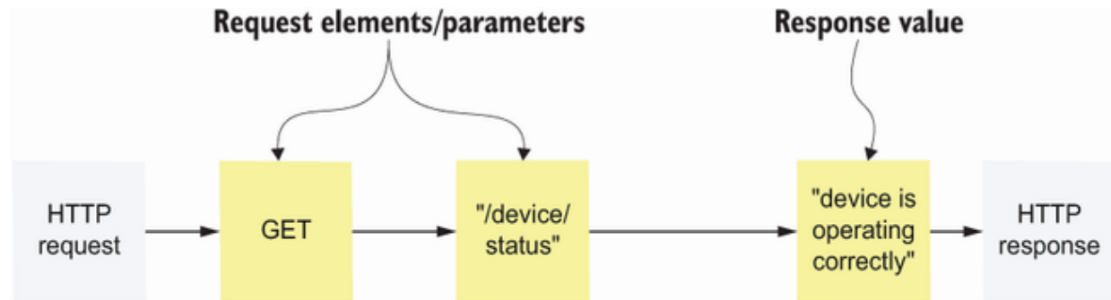
Figure 13.5 Modeling an HTTP request and response in terms of different activities, such as verb, route, and response body. There are, of course, others that would make up such a process, such as setting the status code.
