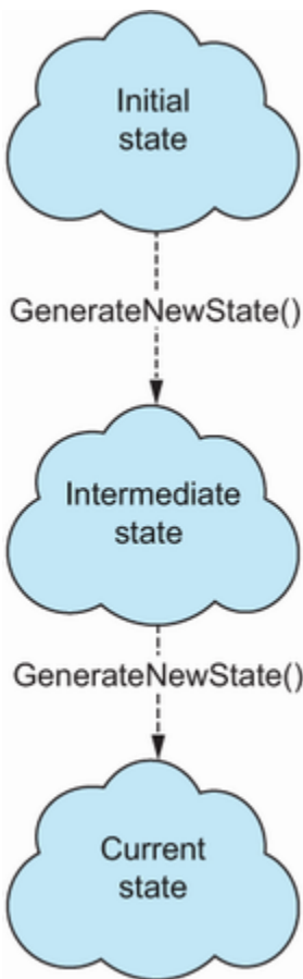
Figure 4.4 Generating new states on every operation with immutable data. Every call to GenerateNewState() creates a new object rather than modifying a single item.
