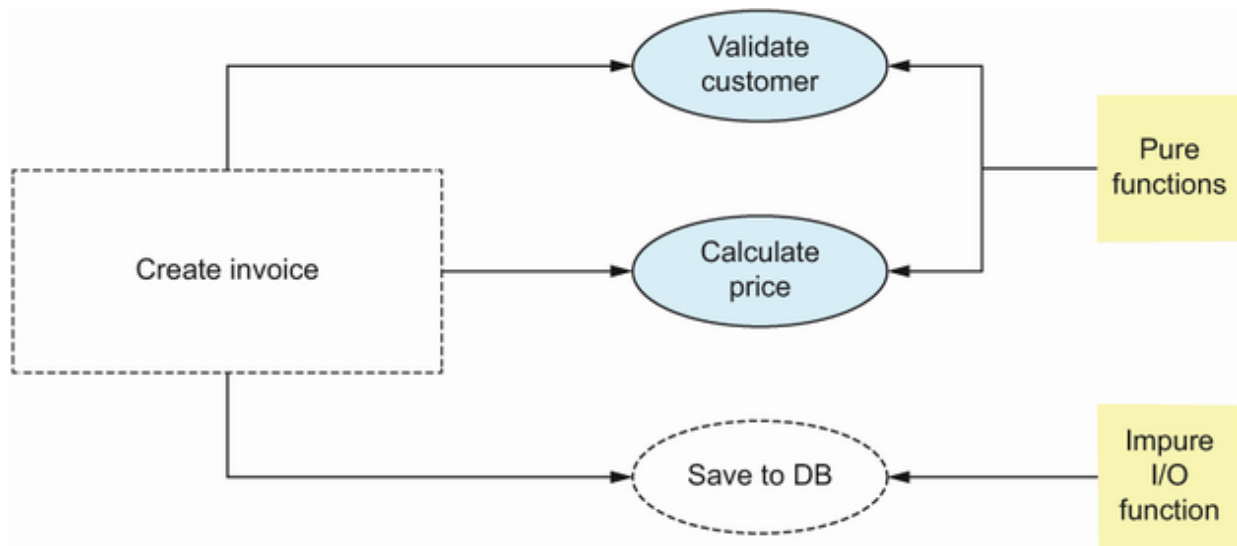
Figure 14.1 A high-level function, Create Invoice, which orchestrates calls to multiple child functions. Validate Customer and Calculate Price in isolation might be good candidates for unit testing as they are pure functions, whereas Save to DB involves I/O and probably wouldn't be a good candidate. This also has a knock-on effect of making Create Invoice impure and I/O-bound; you might instead elect to write an integration test that runs end-to-end, including writing to the database.
