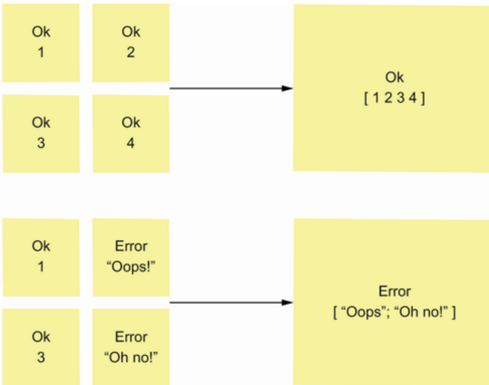
Figure 10.1 Converting a list of result values has two possible outcomes: If all values are ok, the overall result is ok. But if there are any errors, the overall result is an Error.
