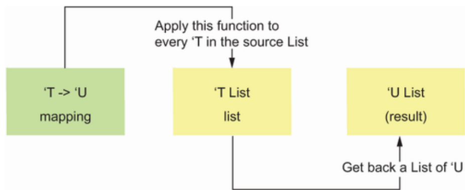
Figure 7.5 The arguments to List.map .
