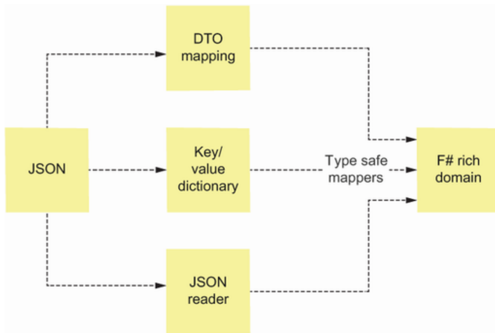
Figure 10.2 Different strategies to safely map from JSON into a rich F# domain model. All utilize some form of intermediate abstraction that allows you to map into F#.
