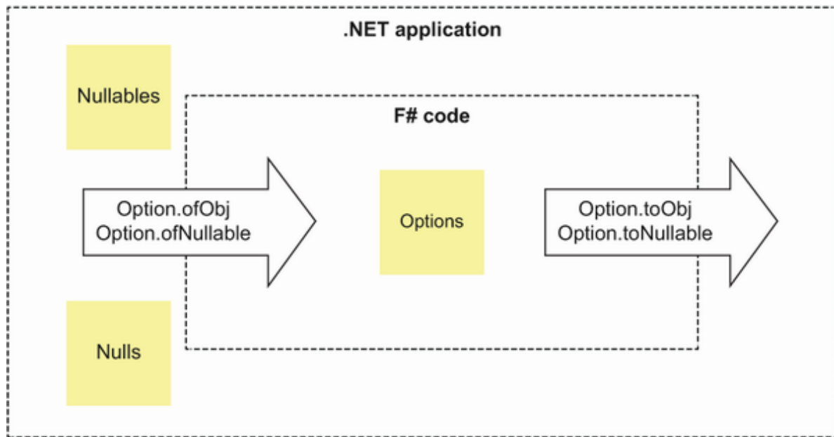
Figure 9.3 When interoperating with non-F# .NET code, using built-in conversion functions in the option module to safely marshal data between options, nulls, and nullables, allowing you to focus solely on using options in your F# code
