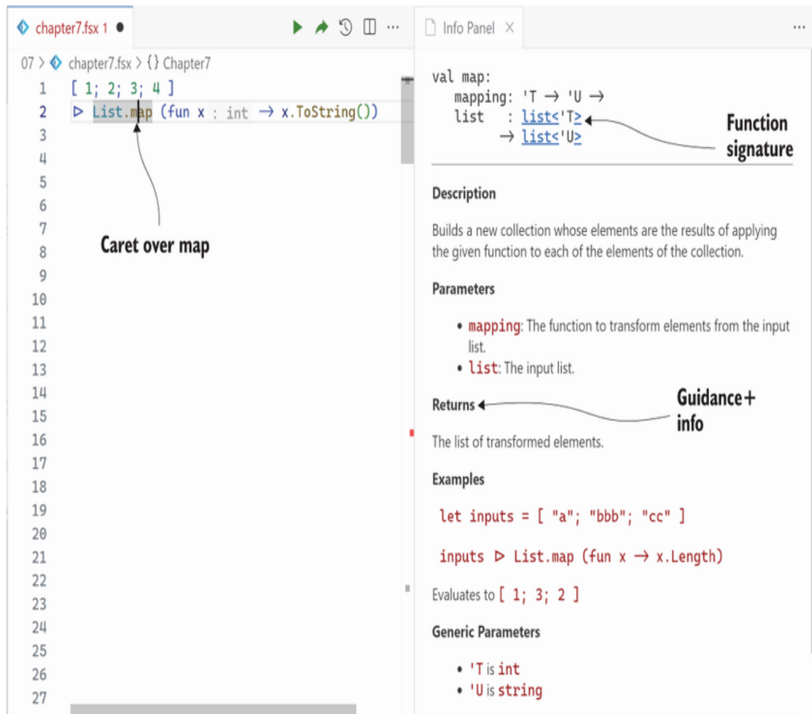
Figure 7.4 VS Code's Info Panel showing help on the List.map function
