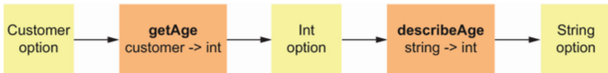
Figure 9.2 A pipeline of operations over optional data
