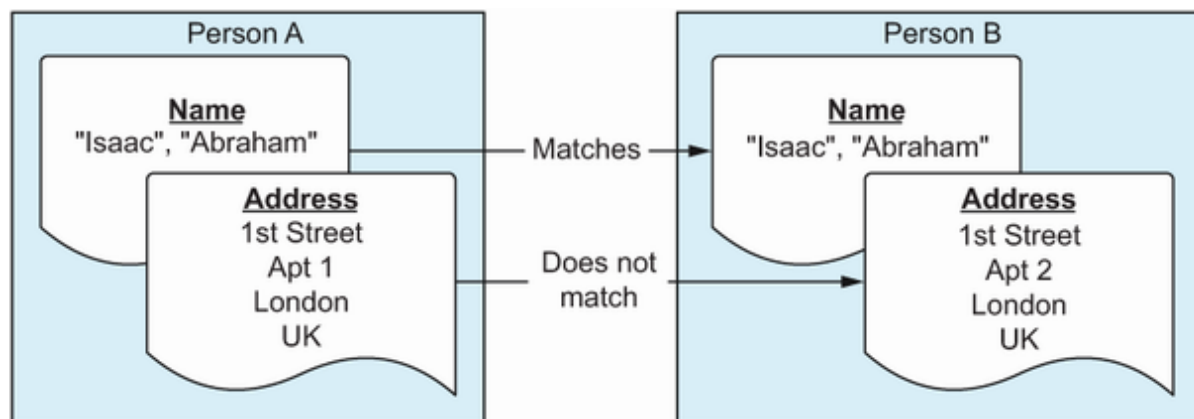
Figure 5.4 F# will perform a deep structural equality check on records. If all fields match, the two records are equal.
