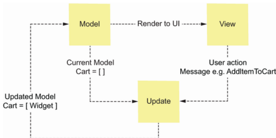
Figure 13.14 The MVU pattern is a pattern that allows you to manage UI changes to a data model in a pure functional style.
