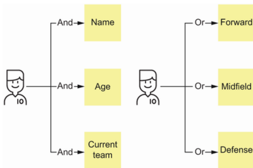
Figure 5.1 Illustrating product (AND) and sum (OR) types. A soccer player has a name, age, and a team, but their position on the field is either forward, midfield, or defense.
