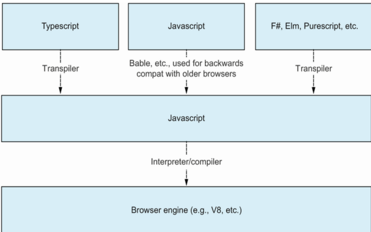
Figure 11.5 The JavaScript language has evolved into a form of an intermediary language that other languages now transpile into to run within the web browser.
