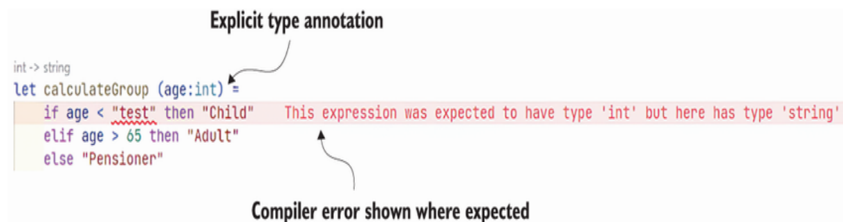
Figure 3.5 Using a temporary type annotation to guide the compiler
