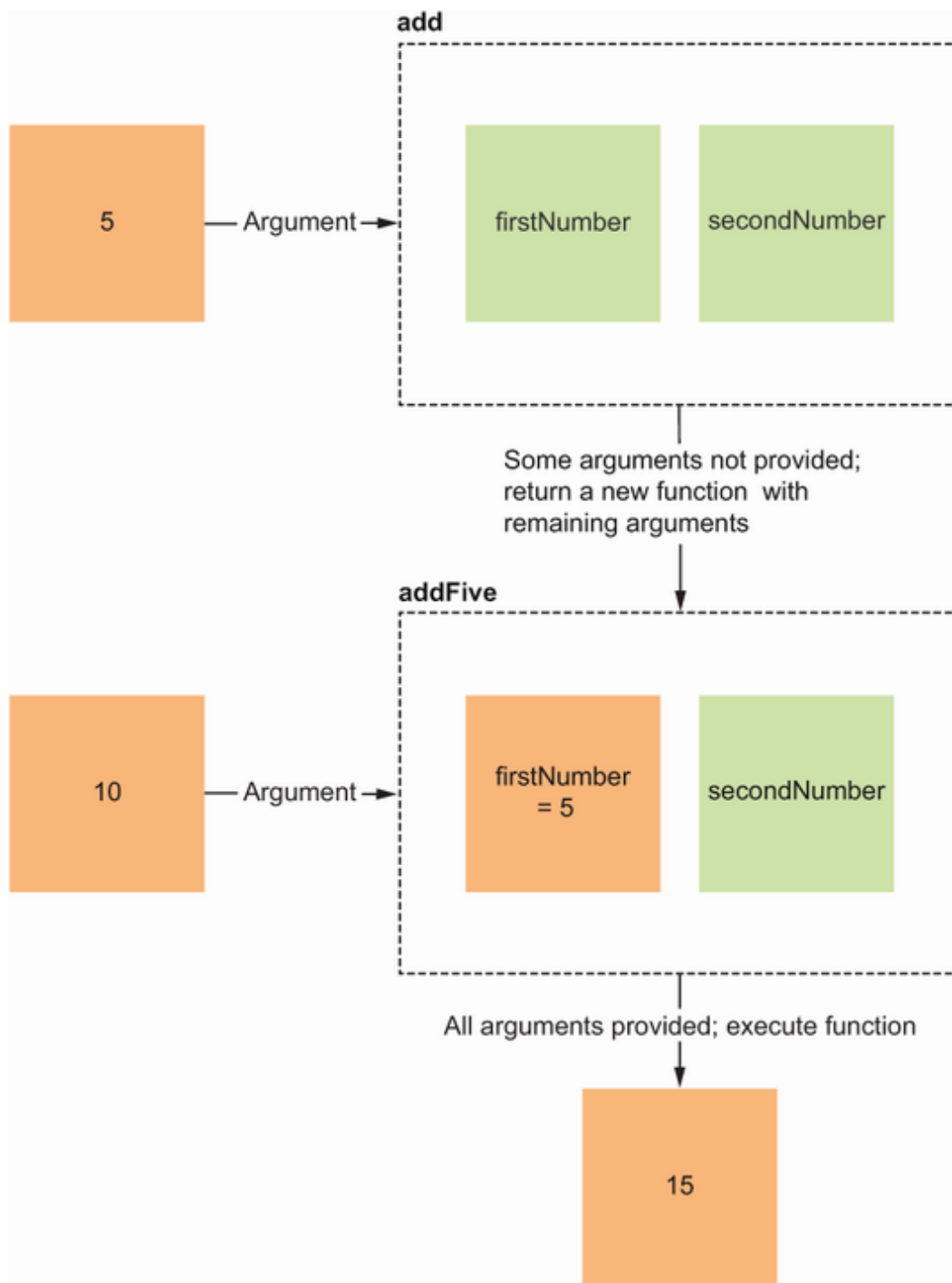
Figure 6.1 Calling an F# function in two stages
