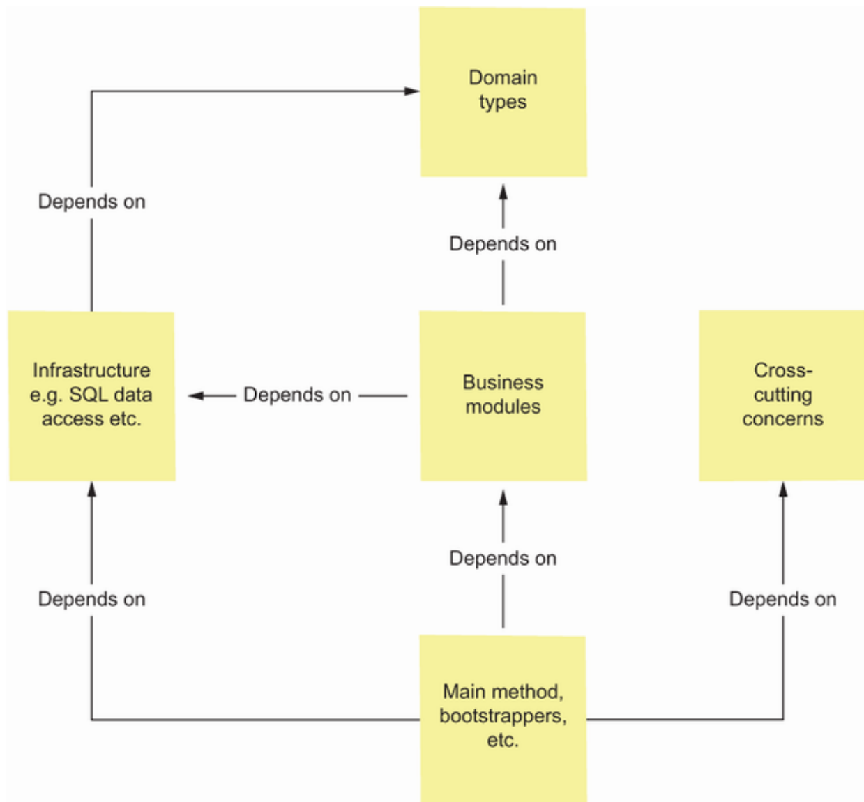
Figure 15.2 A typical dependency graph for types and modules in an F# project
