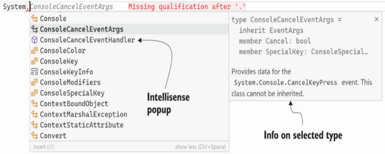
Figure 6.3 Navigating the list of children of the system namespace in VS Code
