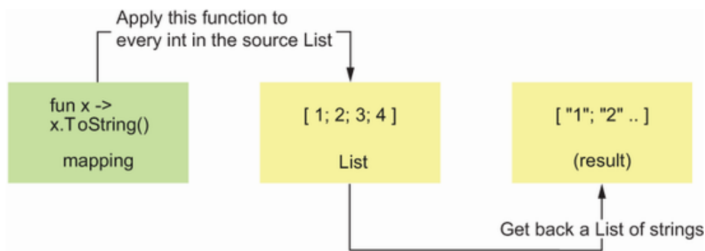
Figure 7.6 The arguments to List.map shown with real values
