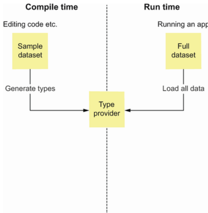
Figure 10.3 Type providers have two distinct phases. At compile time, they are used to create types; at run time, they load in data that meets the previously defined structure.
