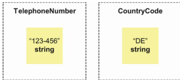
Figure 8.3 Single-case discriminated unions wrap other values to provide richer types. Here, TelephoneNumber and CountryCode are two types that both wrap strings but have different uses and meanings.
