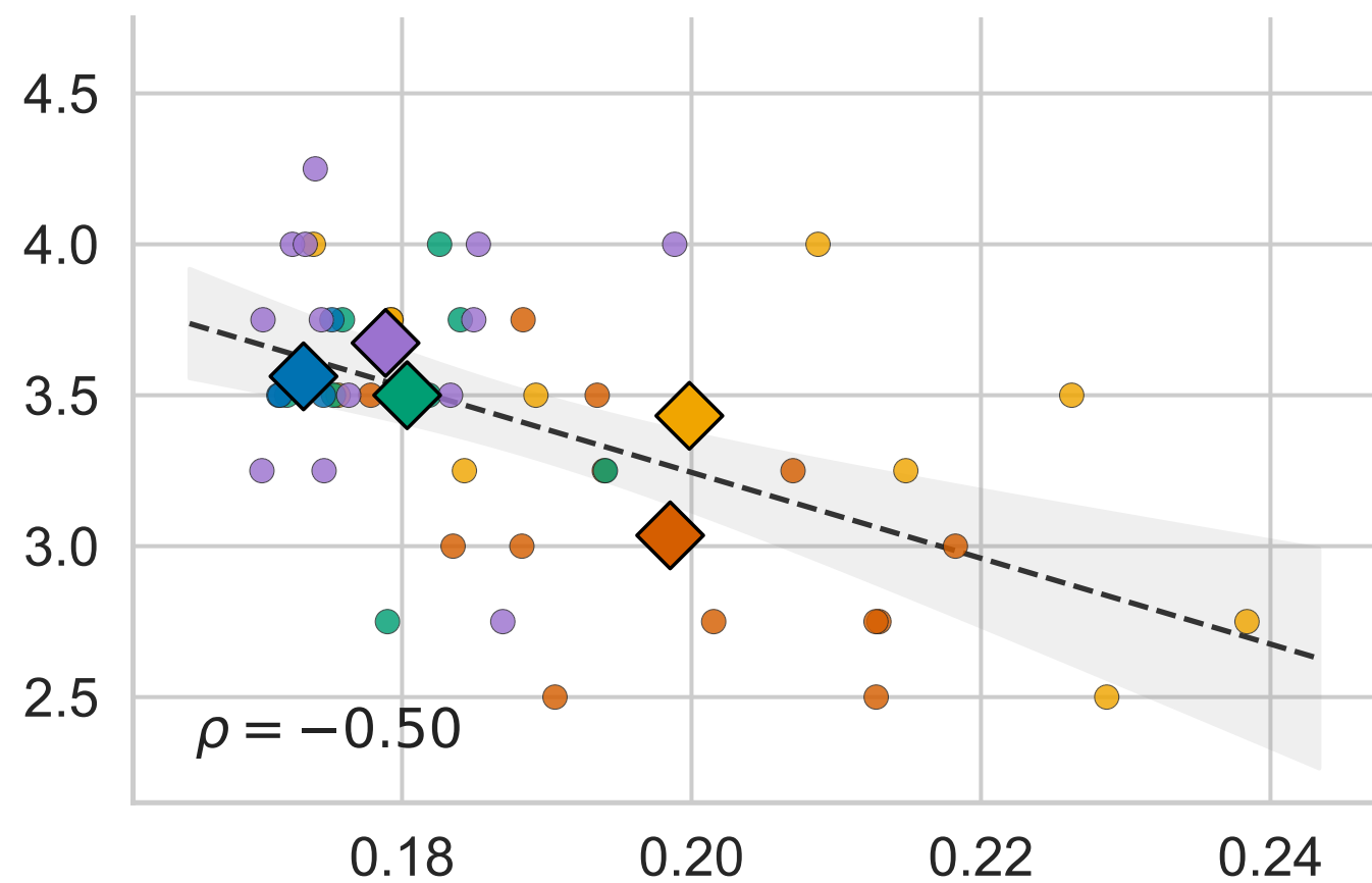
GPT Audio 1.5
