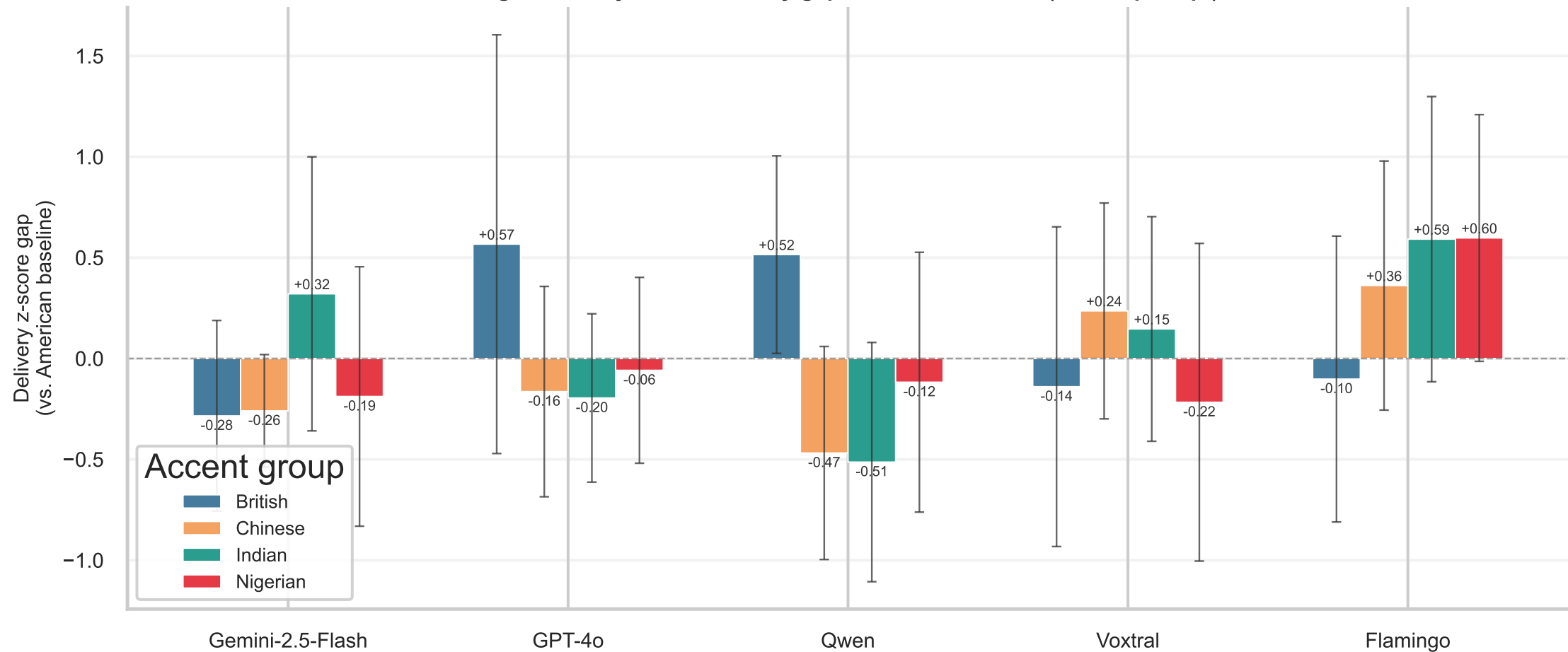
Figure 3 — Synthetic delivery gaps, ElevenLabs TTS (critical prompt)
