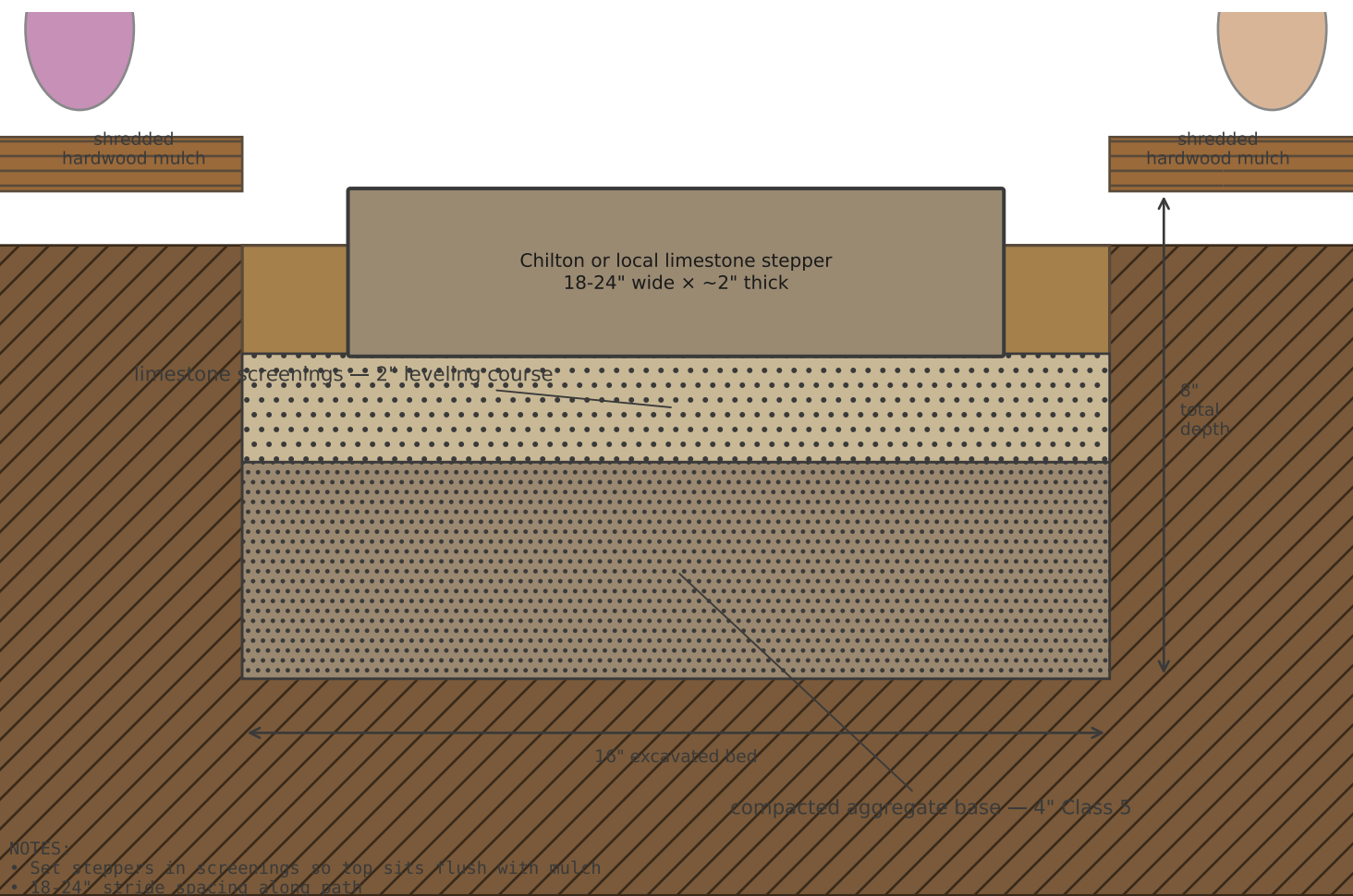
DETAIL 1 — Stepping-Stone Path (scale ~1:8)
