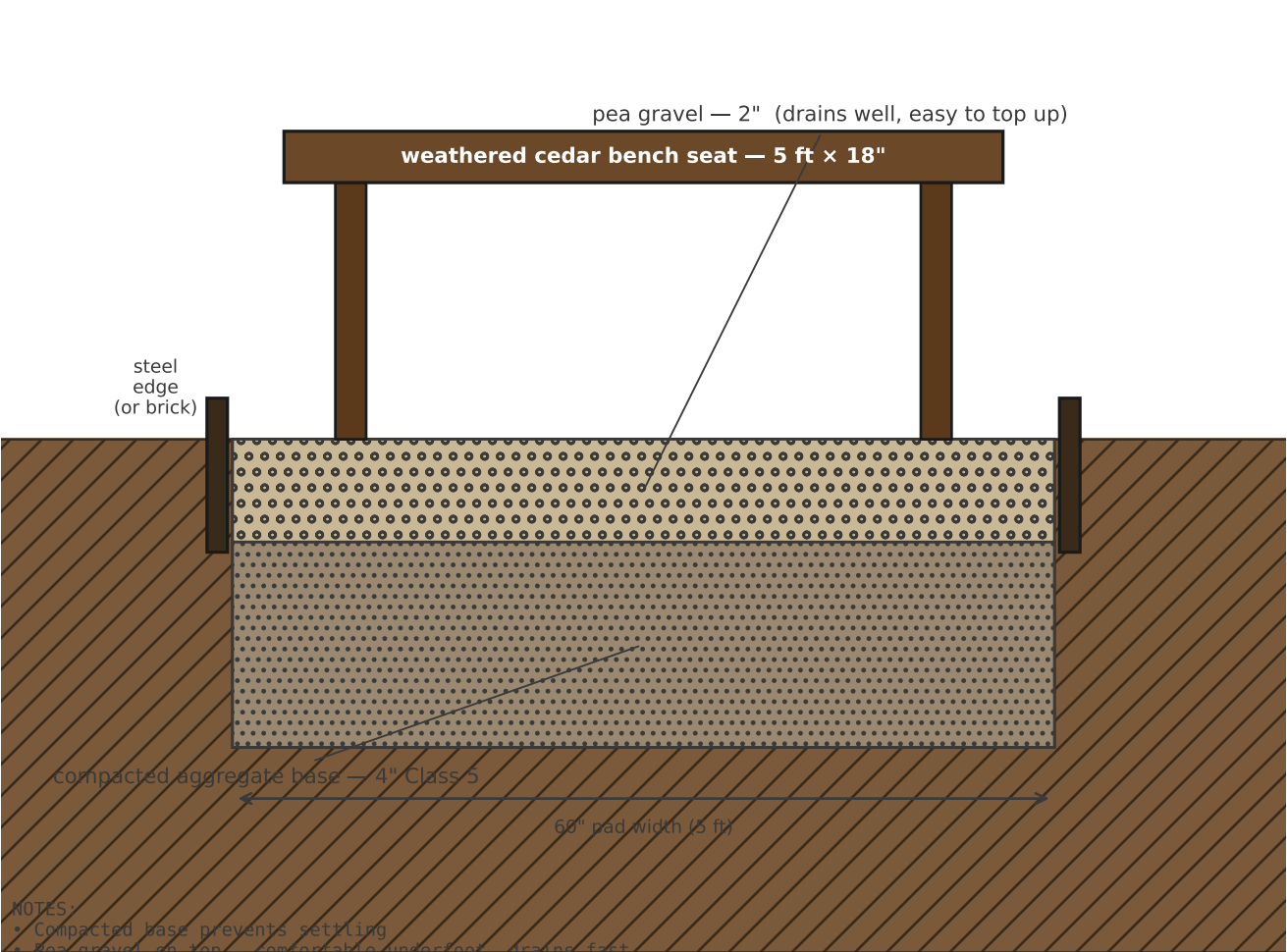
DETAIL 2 — Bench Pad (scale ~1:8)
