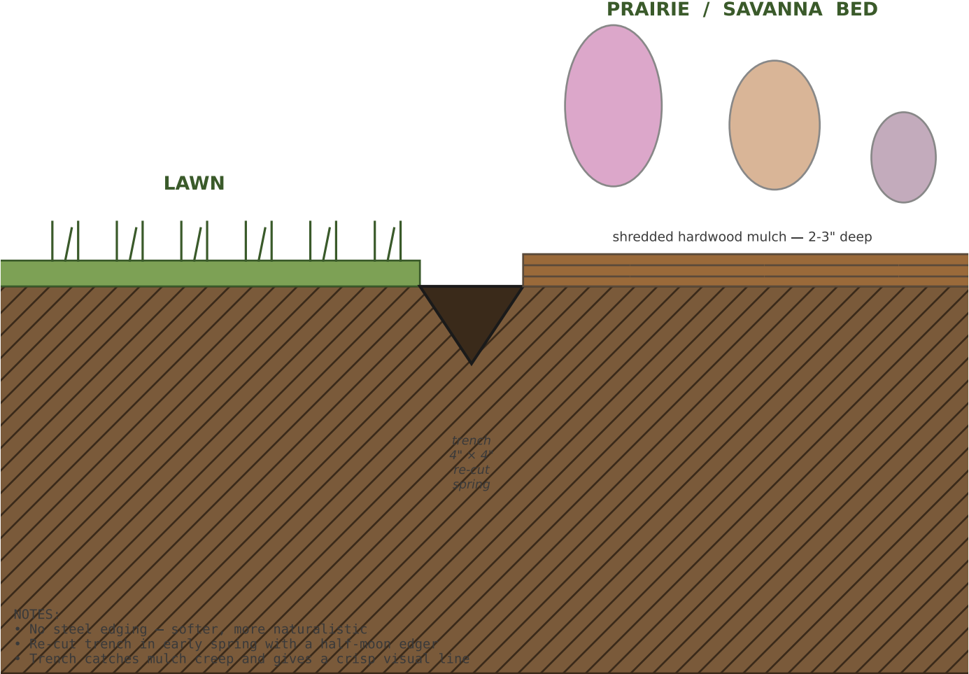
DETAIL 3 — Trench-Cut Bed Edge (scale ~1:4)
