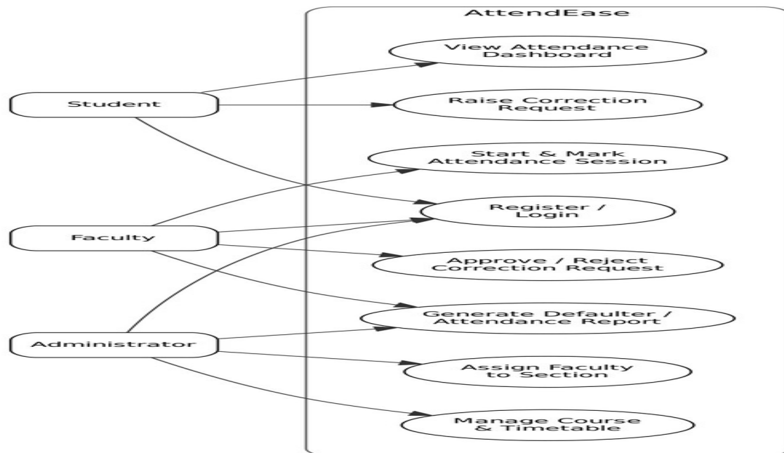
Figure 1: UML Use Case diagram for AttendEase, showing Student, Faculty and Administrator actors against use cases UC-01–UC-08.
