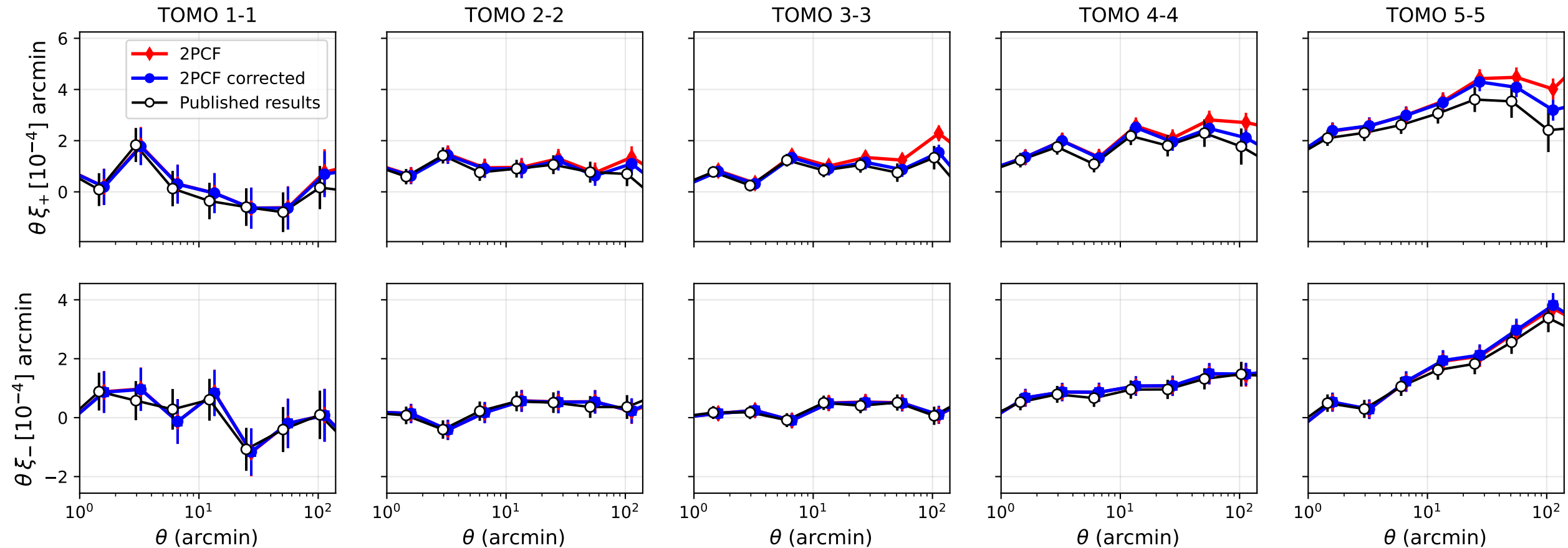
Auto-correlation (2 pt) for the 5 tomographic bins - Published vs calculated
