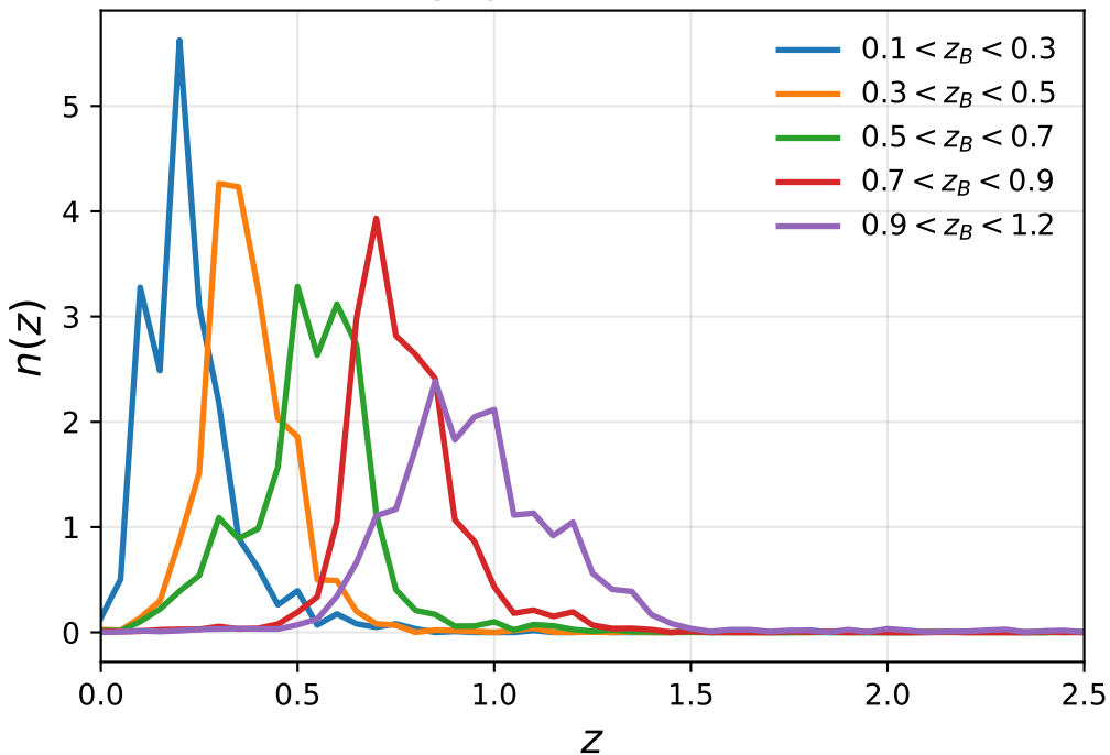
Tomographic bins - KiDS1000
