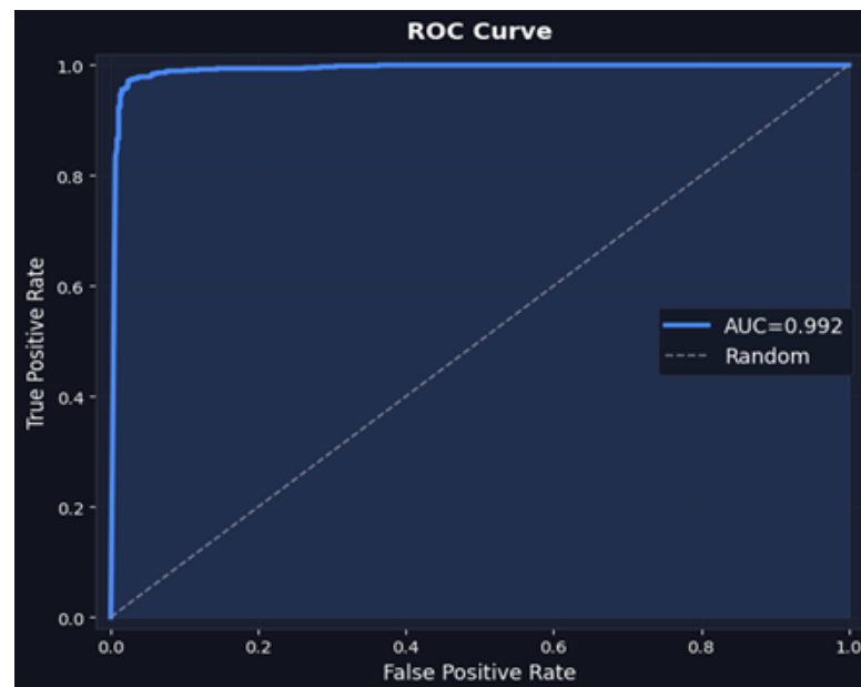
Figure 5.2: Receiver Operating Characteristic (ROC) curve for the proposed hybrid model.
