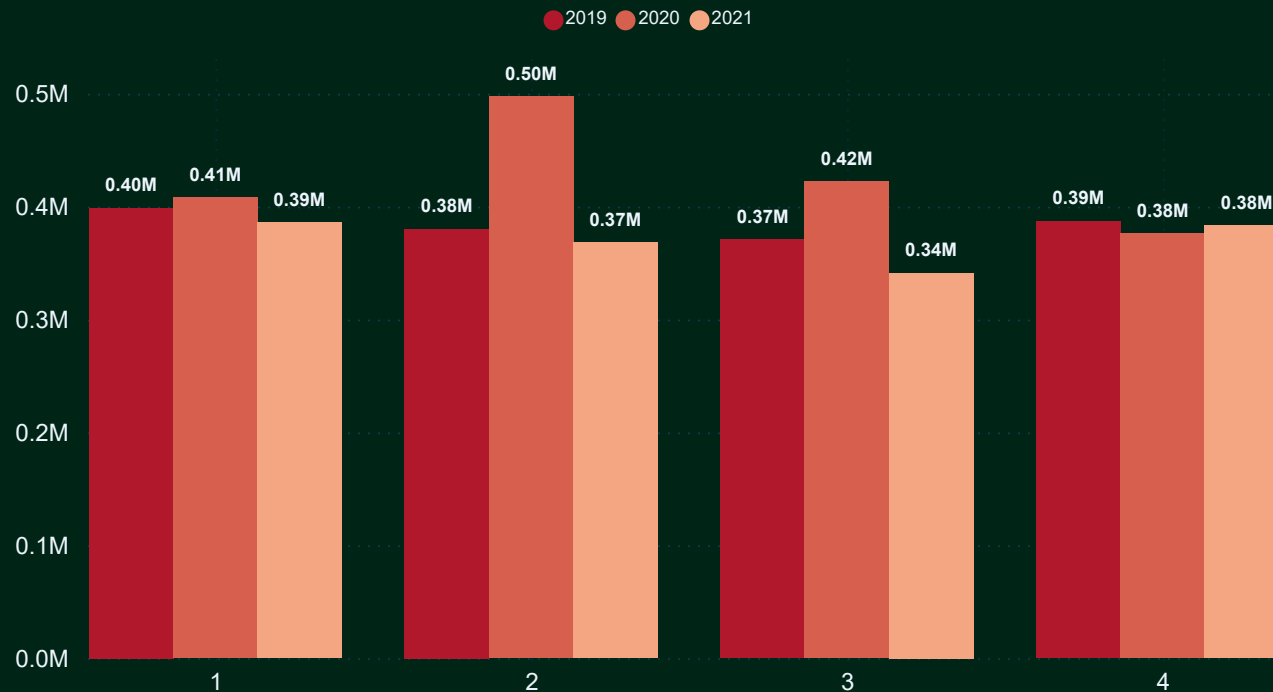
Total Questions by quarter and year
