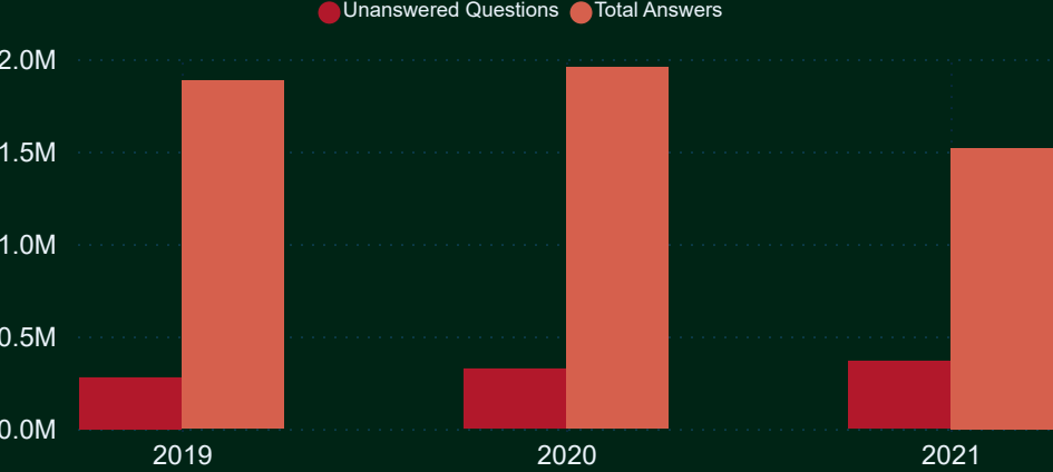
Unanswered Questions and Total Answers by year
