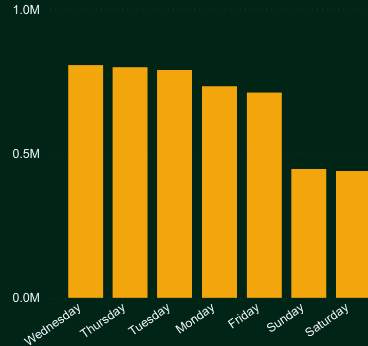
Total Questions by day_name
