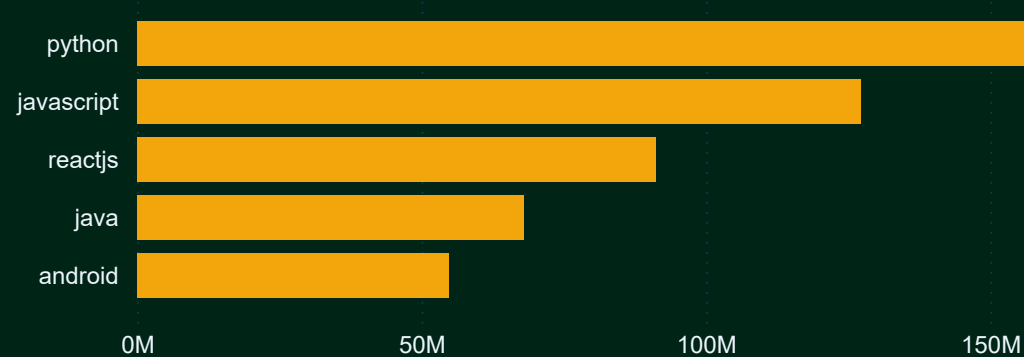
Sum of view_count by tag
