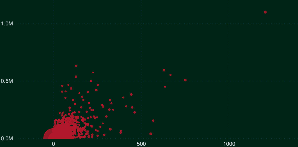
Sum of comment_count by score and view_count
