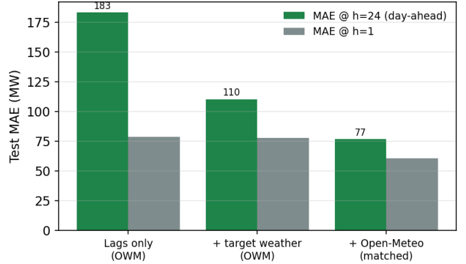
Fig. 2. Day-ahead ( h = 24 ) test-set MAE across the three cumulative configurations: lags-only (183.0 MW) \rightarrow + target-hour weather (110.3 MW) \rightarrow + Open-Meteo train/serve matching (76.7 MW).
