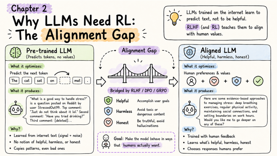
Figure 2.1: The alignment gap – from a pre-trained LLM that predicts tokens to an aligned assistant that is helpful, harmless, and honest.
