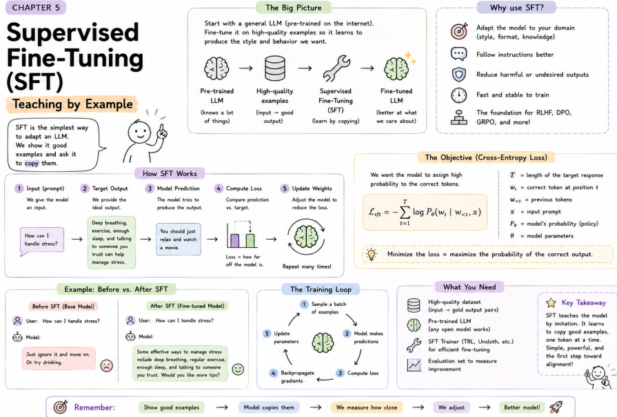
Figure 5.1: Supervised fine-tuning at a glance – from pre-trained LLM to fine-tuned model via high-quality examples and cross-entropy loss.
