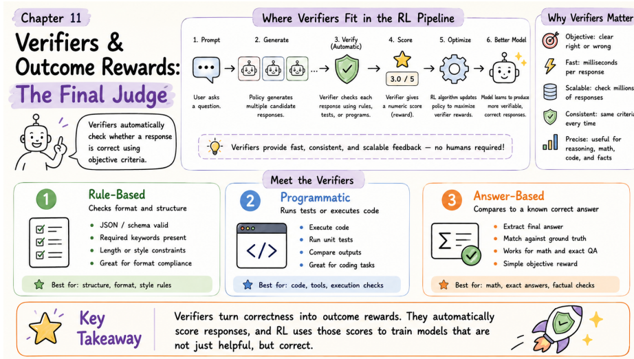
Figure 11.1: Verifiers and outcome rewards at a glance — when scores come from automatic checks instead of learned models.
