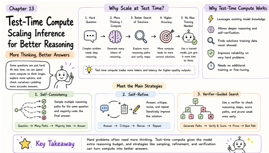
Figure 13.1: Test-time compute at a glance – spend extra computation per query to produce better answers without retraining the model.
