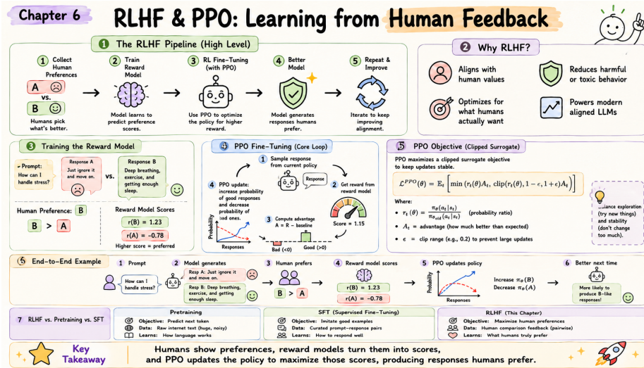
Figure 6.2: RLHF and PPO in depth – the full pipeline from preference data through reward model training, PPO objective, and end-to-end alignment.
