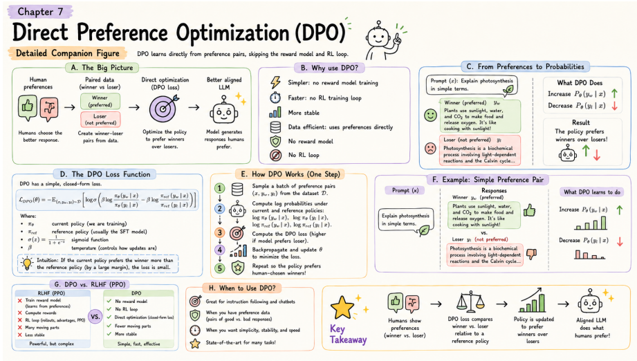
Figure 7.2: DPO in depth – the full derivation from preference pairs through the reparameterization trick, loss function, and comparison with RLHF.
