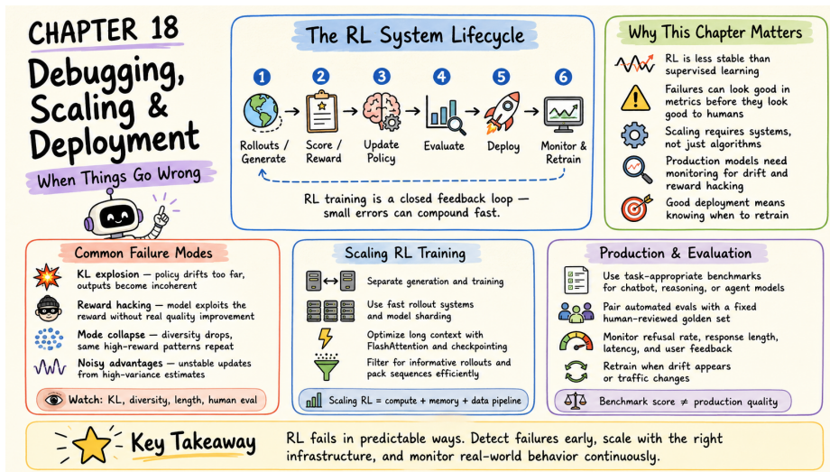
Figure 18.1: Debugging, scaling, and deployment at a glance – failure modes, scaling techniques, and production evaluation across the RL system lifecycle.
