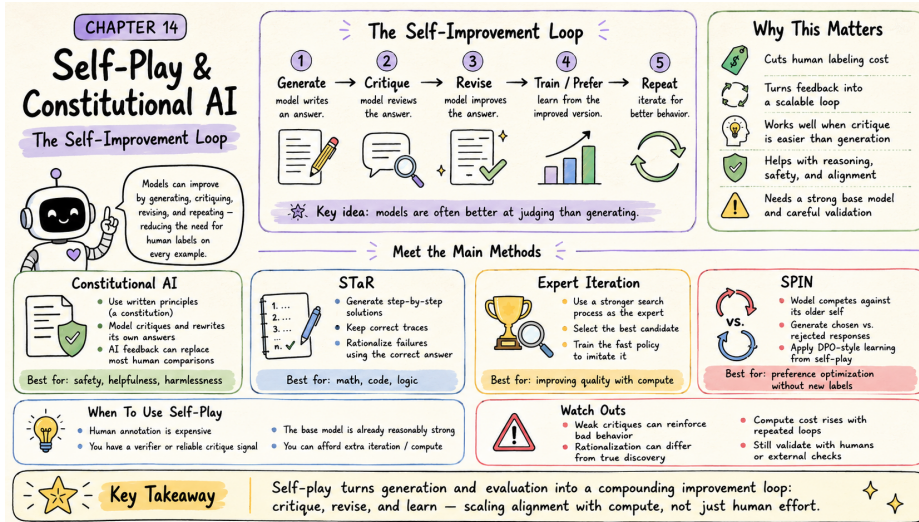
Figure 14.1: Self-play and Constitutional AI at a glance – the self-improvement loop and the main methods that exploit the verify-easier-than-generate asymmetry.
